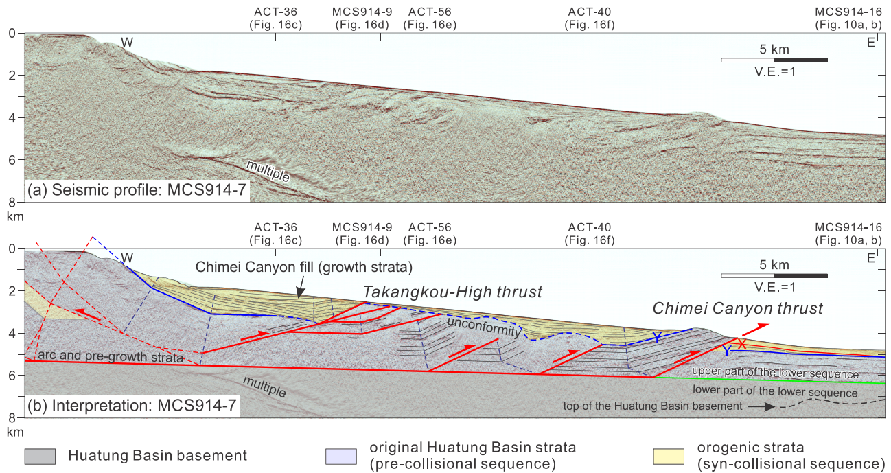
Figure 15. (a) Prestack depth migrated short-streamer seismic profile MCS914-7 along the Chimei Canyon. The profile shows tilted pregrowth strata (lower seismic sequence, purple) and slightly deformed growth strata (middle and upper seismic sequence, yellow). The frontal thrust is best imaged in this profile and defines the lower limit of the Chimei Canyon. (b) Seismic interpretation. The red solid lines are the thrusts and detachment. Red dashed lines are less certain thrusts. The west-vergent structures at the west end of the profile, which are thought to be responsible for the steep headwall of Chimei Canyon, are interpreted from surface geological data onshore Coastal Range (see Figure 17). See Figure S7 for higher resolution images.
