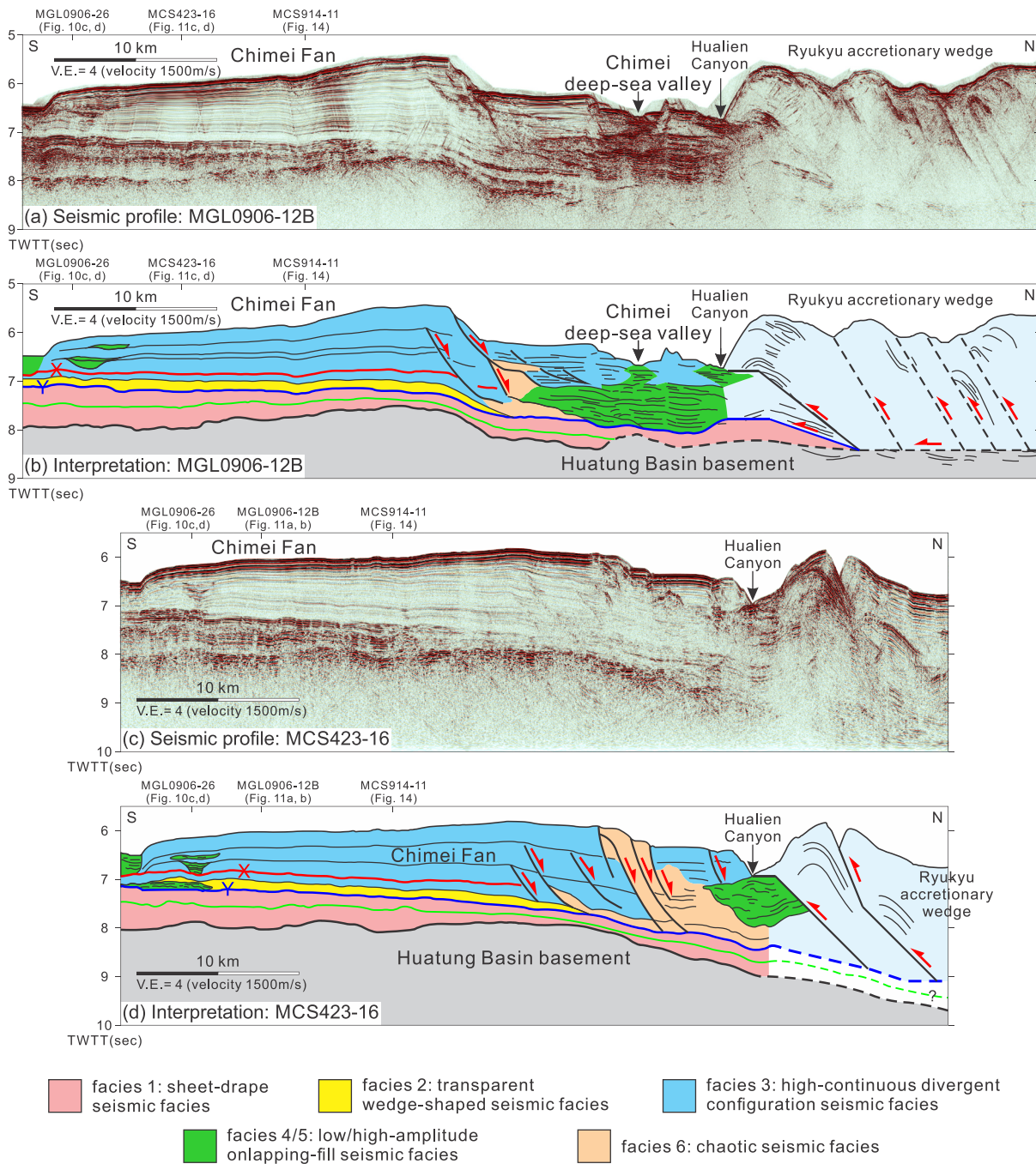
Figure 11. (a) Seismic profile of the Chimei fan and deep-sea valley: MGL0906-12B. This seismic profile shows that the Chimei Fan and deep-sea valley are beginning to be incorporated into the Ryukyu accretionary wedge. (b) Seismic interpretation of (a). (c) Lower fan seismic profile of the Chimei Fan: MCS423-16. This seismic profile is the easternmost profile across the Chimei Fan (see Figure 6 for location). The canyon in this profile is the Hualien Canyon because the Chimei deep-sea channels merged into the Hualien Canyon west of this seismic profile. See Figures S4 and S5 for high-resolution versions of these profiles.
