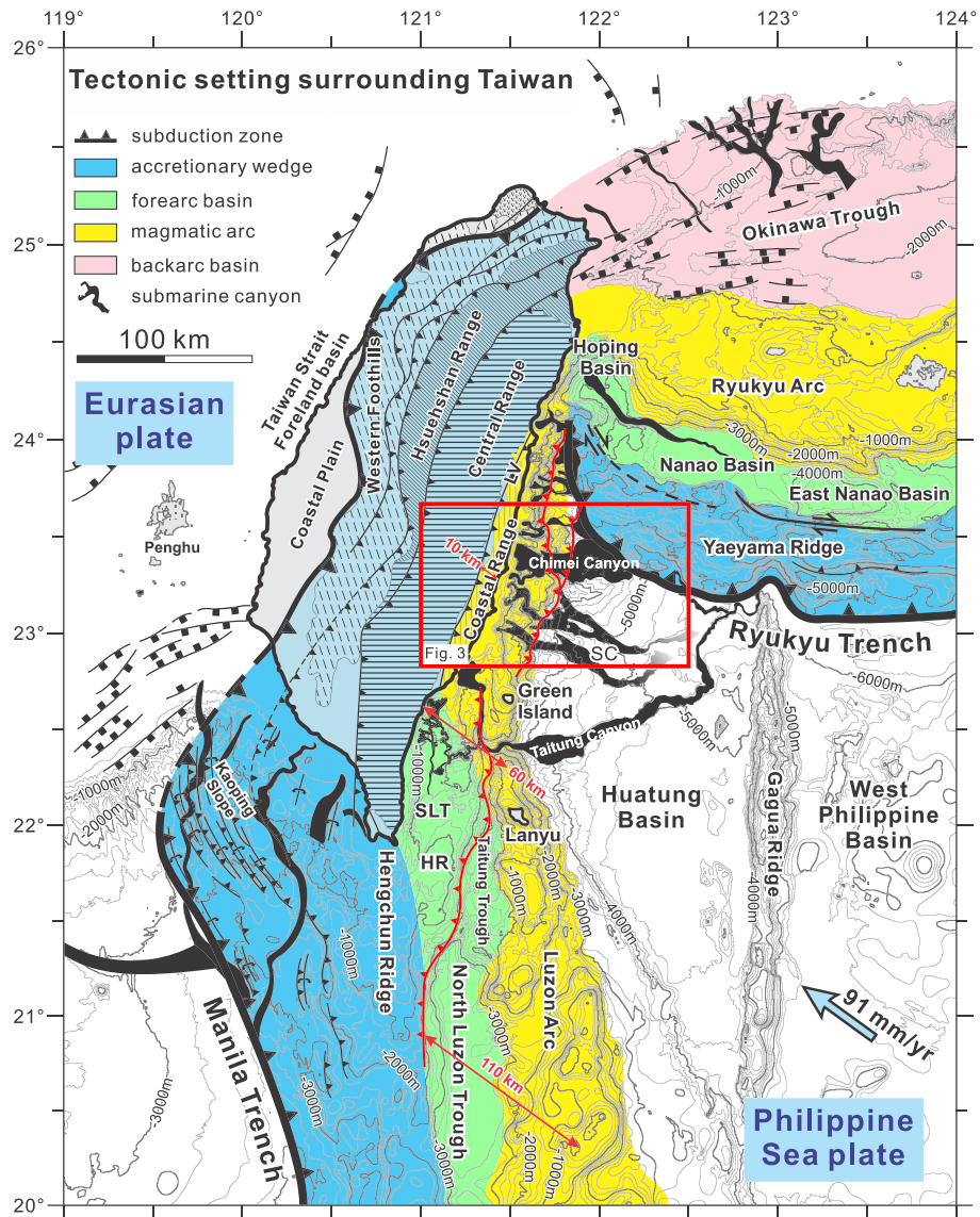
Figure 2. Tectonic setting of Taiwan, showing surrounding submarine canyons that currently transport orogenic sediment into deep ocean basins. The Taiwan arc-continent collision is located at the junction of two orthogonal subduction zones: The NS Manila subduction zone in the south extending to northern Taiwan and the EW Ryukyu subduction zone in the northeast, with associated Okinawa Trough backarc basin. The colors show tectonic elements (blue: accretionary wedge, green: forearc basin, yellow: magmatic arc, and red: backarc basin). SLT = Southern Longitudinal Trough; HR = Huatung Ridge; LV = Longitudinal Valley; SC=Sanxian Canyon. The offshore structures are from Liu et al. (2004) and submarine canyons from Chiang and Yu (2006), Hsiung and Yu (2011), and Yang (2001). The forearc basin is ~110 km wide in the south, measured in the plate convergence direction but is increasingly compressed northward during oblique arc-continent collision, becoming only ~10 km in the Taiwan Coastal Range.
