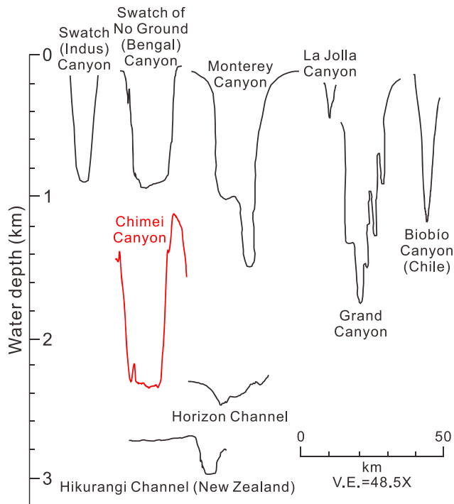
Figure 1. Comparison of Chimei Canyon in cross section with well-known submarine canyons in convergent-margin settings (except Grand Canyon). Vertical axis shows water depth. This figure is modified from Normark and Carlson (2003): Swatch Canyon (Shepard, 1973); Swatch of No Ground Canyon (Curray & Moore, 1974; Shepard, 1973); Monterey Canyon and Grand Canyon (Carlson & Karl, 1988); La Jolla Canyon (Shepard & Buffington, 1968); Biobio Canyon (Bernhardt et al., 2015); Horizon Channel (Stevenson & Embley, 1987); Hikurangi Channel (Mountjoy et al., 2018).
