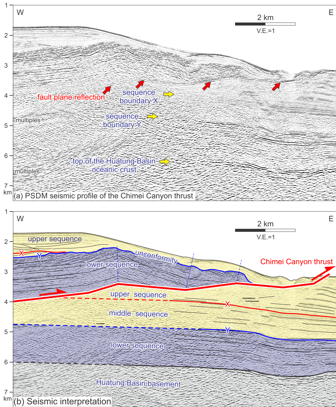
Figure 13. Detail of prestack depth migrated short-streamer seismic profile MCS914-11 (Figure 14), along the southern Chimei Canyon wall, imaging the Chimei Canyon thrust. The map location is shown in Figure 4.
