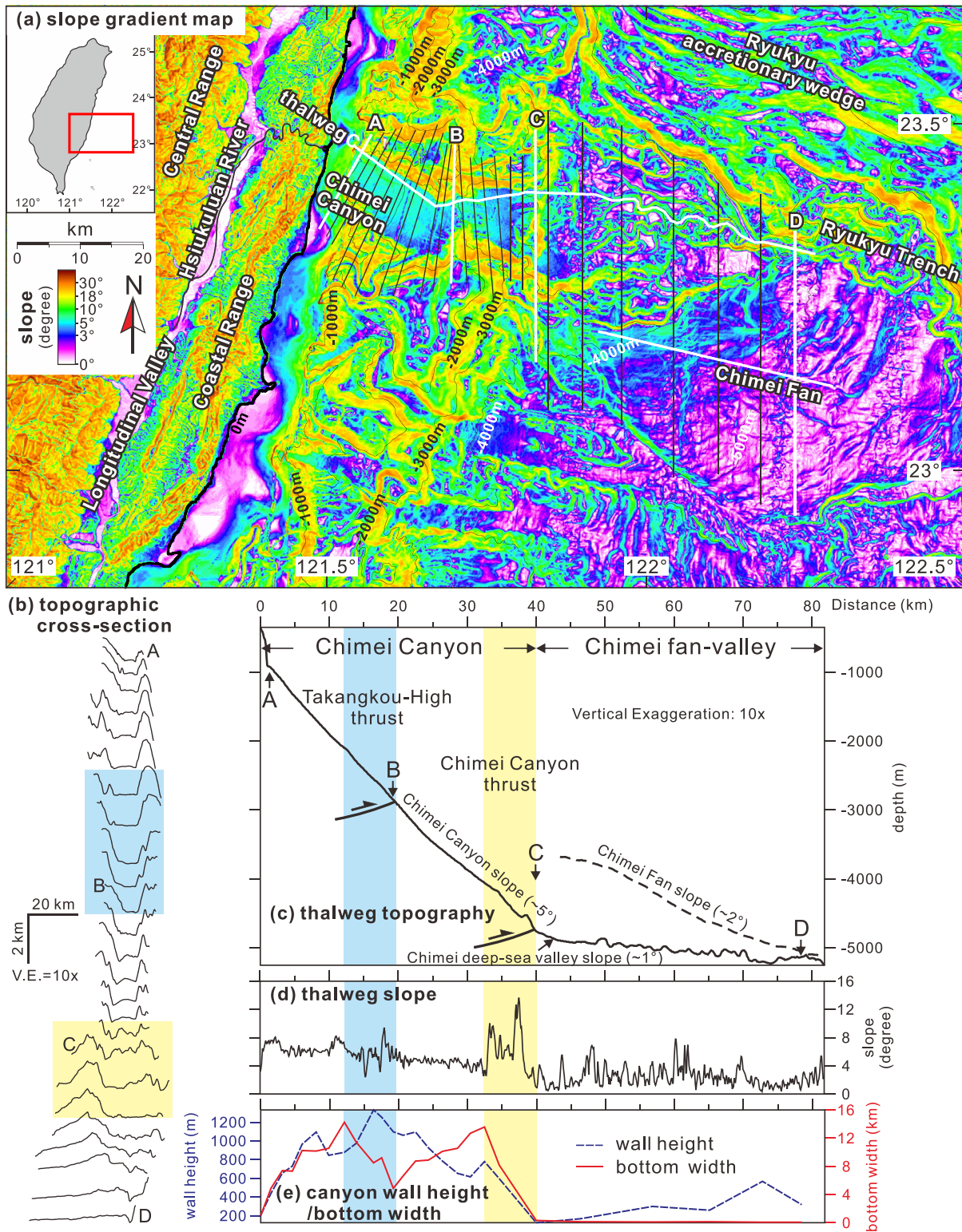
Figure 7. (a) Slope gradient map of the Chimei Canyon-Fan system. (b) Topographic cross sections of the Chimei Canyon-Fan system from upstream to downstream. The locations of cross-sections are shown in (a), with four profiles marked by A–D. (c) Canyon, deep-sea channel thalweg, and fan topography. (d) Slope gradient along the Chimei Canyon and deep-sea channel thalweg. (e) Height of the canyon/deep-sea channel walls and width of the canyon/deep-sea channel bottom. Two active thrust zones with associated folding are shown by blue and yellow background.
