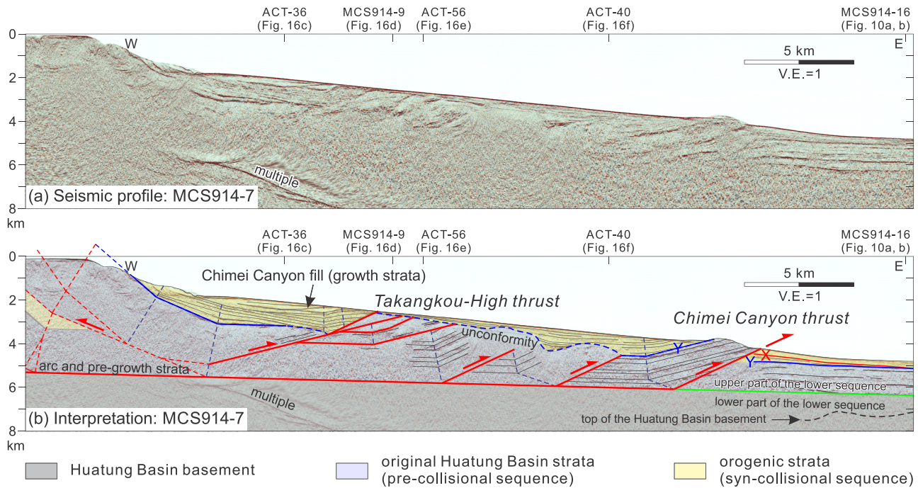
Figure 15. (a) Prestack depth migrated short-streamer seismic profile MCS914-7 along the Chimei Canyon. The profile shows tilted pre-growth strata (lower seismic sequence, purple) and slightly deformed growth strata (middle and upper seismic sequence, yellow). The frontal thrust is best imaged in this profile and defines the lower limit of the Chimei Canyon. (b) Seismic interpretation. The red solid lines are the thrusts and detachment. Red dashed lines are less certain thrusts. The west-vergent structures at the west end of the profile, which are thought to be responsible for the steep headwall of Chimei Canyon, are interpreted from surface geological data onshore Coastal Range (see Figure 17). See Figure S7 for higher resolution images.
