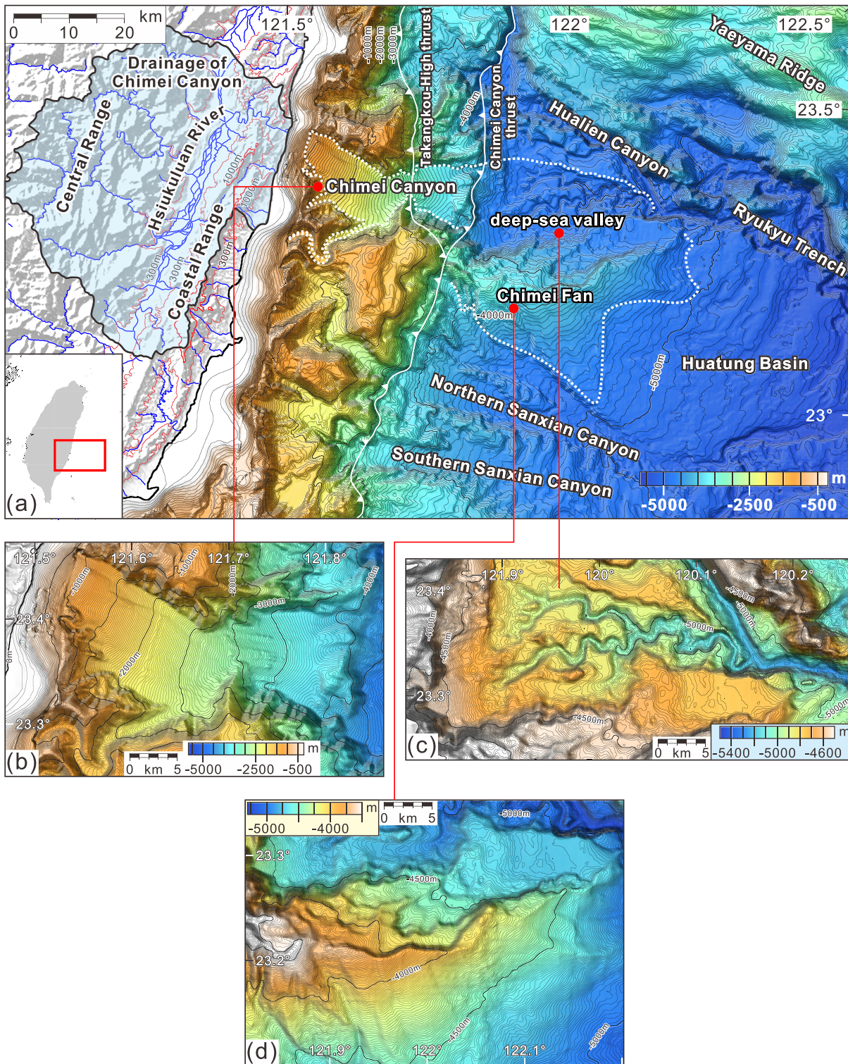
Figure 3. Detailed bathymetric map of the Chimei Canyon-Fan system (see location in Figure 2). Note that the depth range of the color scale is compressed in (c) and (d) to illuminate the low-relief deep-water morphologies. (a) Overview of the Chimei Canyon-Fan system. The outline of the canyon and fan is shown with white dots. The Chimei Canyon thrust lies at the foot of the slope, separating the canyon and deep-sea valley. The Takangkou High thrust cuts across the middle of the Chimei Canyon. Rivers onshore are shown by light blue lines and the Hsiukuluan River catchment (source of the Chimei Canyon-Fan system) is shown by light blue area. (b) Detailed bathymetric map of the Chimei Canyon showing a wide and smooth canyon bottom. (c) Detailed bathymetric map of the Chimei deep-sea valley. (d) Detailed bathymetric map of the Chimei Fan which shows the preserved southern part of the fan and erosional features in the northern part of the fan.
