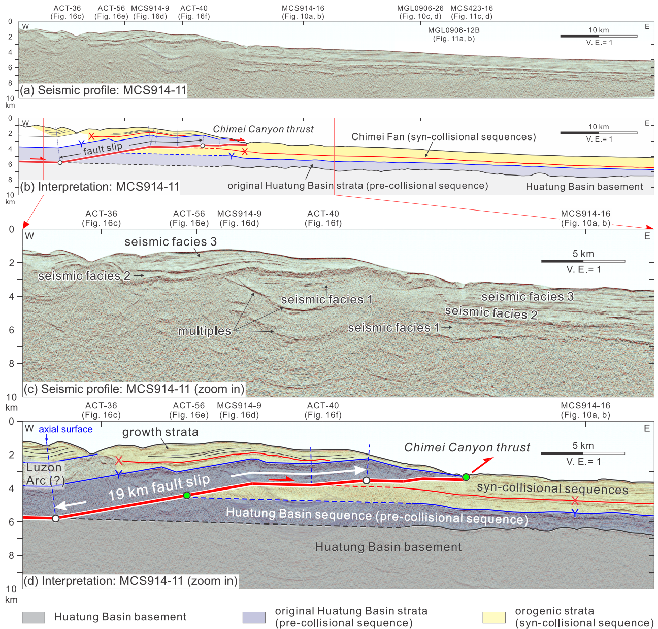
Figure 14. (a) Prestack depth migrated short-streamer seismic profile MCS914-11 along the southern Chimei Canyon wall and Chimei Fan. This seismic profile shows that the Chimei Fan has been uplifted by the Chimei Canyon thrust. A detail of the section at the toe of the thrust is shown in Figure 13. (b) Seismic interpretation. (c) Zoom in part of the seismic profile (a) and its interpretation (d). See Figure S6 for higher-resolution images.
