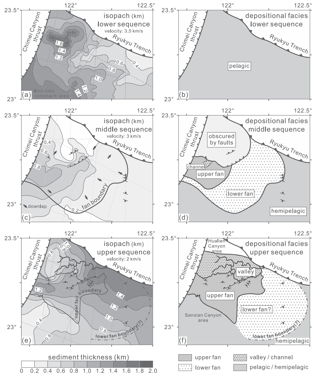
Figure 12. (a, c, and e) Isopach and (b, d, and f) distribution of seismic facies assemblage of the three seismic sequences east of the Chimei Canyon thrust. The thickness of seismic sequence is calculated based on the average velocity of each seismic sequence, which is obtained by the velocity analysis of seismic CMP gathers (applied velocity is shown in each figure).
