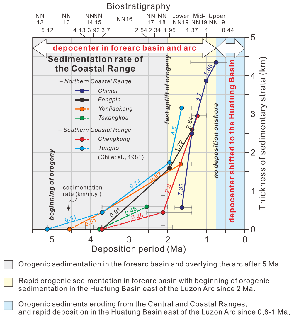
Figure 5. The sedimentation rate for stratigraphic sections of the Coastal Range (updated from Chi et al., 1981, using timescale of Cohen & Gibbard, 2019). The sedimentation rates increase abruptly around 2 Ma and sedimentation terminates \leq 1 Ma. Different outcrop sections are shown by different colors. Values along each line show the average sedimentation rate in km/my. Gray lines are the error bars for age.
