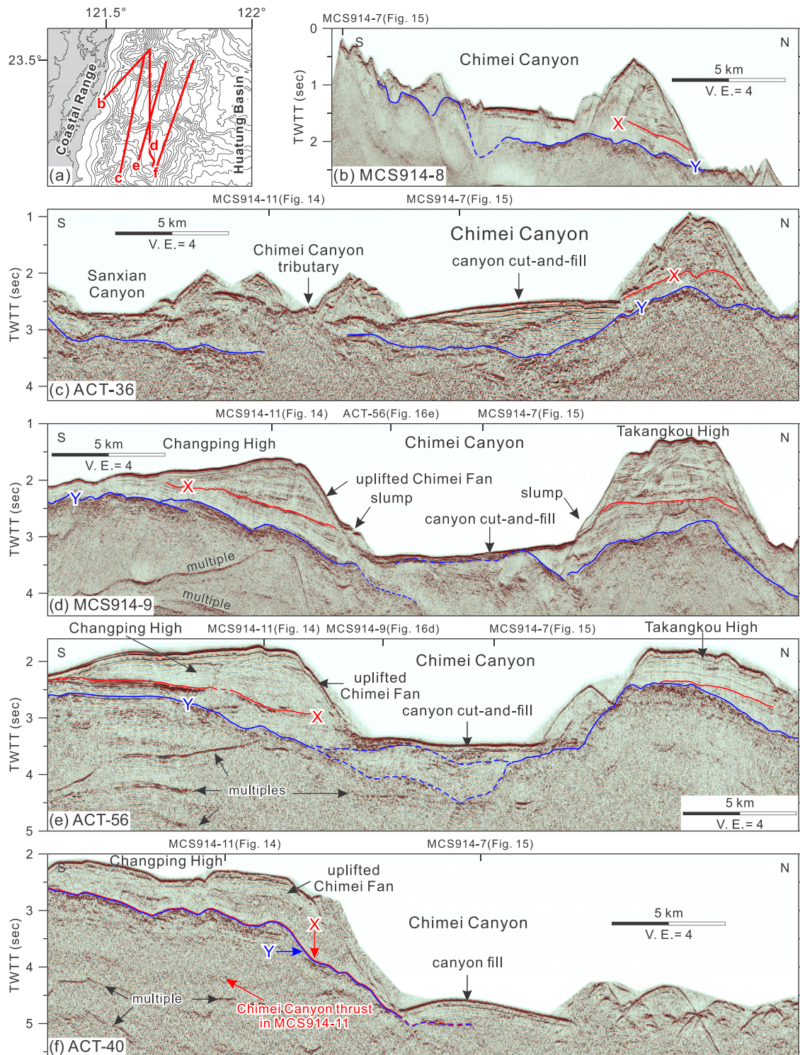
Figure 16. Seismic profiles across the Chimei Canyon from upstream to downstream. Location of each seismic profile is shown in (a). Two seismic sequence boundaries X and Y are shown.
