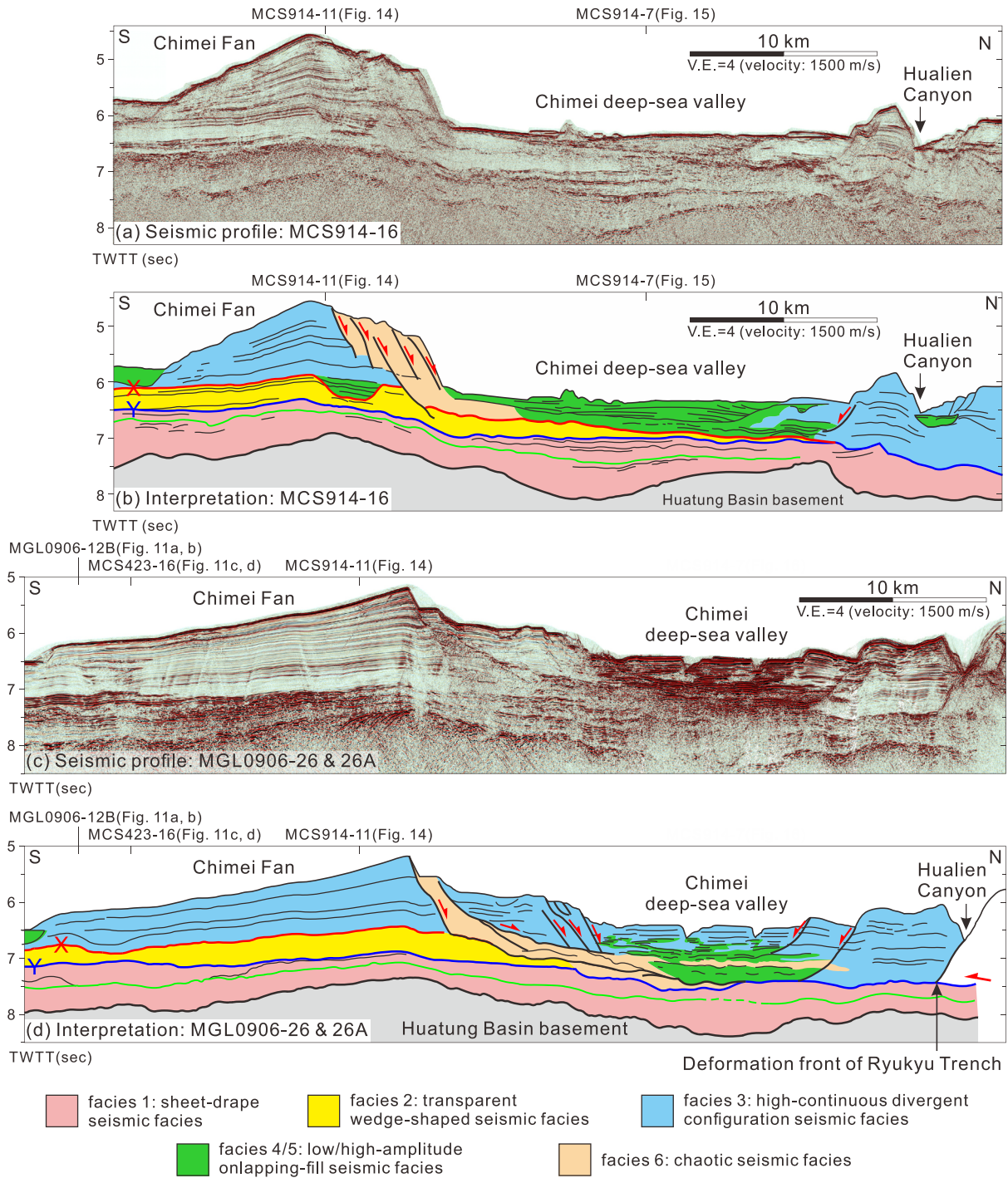
Figure 10. Upper fan seismic profiles of the Chimei Fan. (a) Seismic profile MCS914-16. This seismic profile is the closest profile to the canyon (see Figure 6 for location). (b) Seismic interpretation of (a). (c) Seismic profile MGL0906-26 and 26A. (d) Seismic interpretation of (c). X and Y are seismic sequence boundaries. Colors show the seismic facies. Locations of crossing seismic profiles are given by tick marks. See Figures S2 and S3 for high-resolution versions of those profiles.
