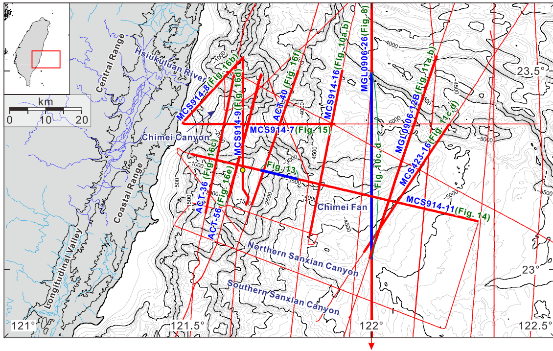
Figure 6. Location map showing the seismic reflection profiles used in this study. Bold lines are the seismic profiles shown in this paper. Yellow dot is the location of the marine core (Lallemand et al., 2016; Lehu et al., 2016).
