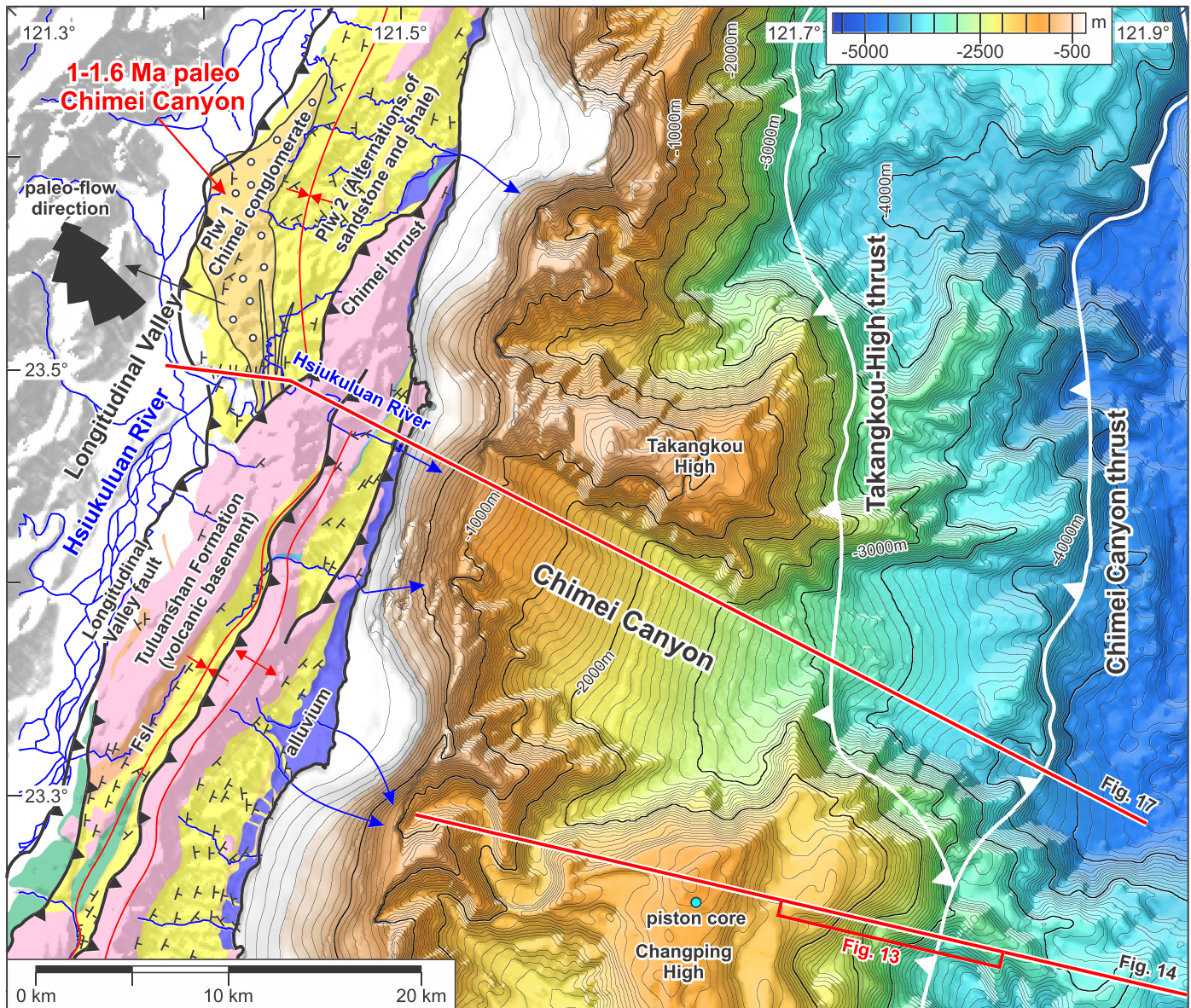
Figure 4. Combined geological map of the Coastal Range and bathymetric map offshore eastern Taiwan. The thin-skinned west-vergent Coastal Range thrust belt deforms arc and forearc basin strata, including paleo-submarine canyon and fan strata (Fanchuliao [Fsl] and Paliwan Formation [Plw1 and Plw2]) together with Luzon Arc (Tuluanshan Formation) uplifted to 1,000- to 1,500-m elevation, whereas the offshore Chimei Canyon has undergone east-vergent thrust deformation. The 1- to 1.6-Ma Chimei conglomerate exposed onshore is interpreted as a paleo-Chimei Canyon deposit, which shows a similar paleo-flow direction to the present-day upper Chimei Canyon (Dorsey & Lundberg, 1988). A cross section along the current transport pathway is shown as Figure 17. The geological map of Coastal Range is based on data from Wang and Chen (1993) and Shyu et al. (2006).
