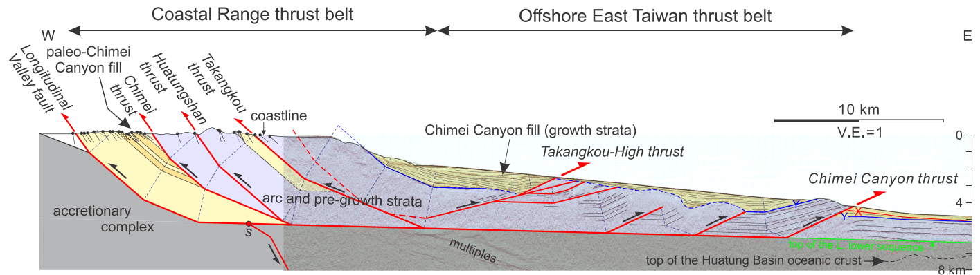
Figure 17. Combined onshore-offshore structural section along the wedge-top Hsiukuluan River-Chimei Canyon transport pathway (Figure 4). The shortening is \geq 60 km, which is largely post 1 Ma and is consistent with present-day \sim 60 mm/yr geodetic shortening rate. The eastern limit of Chimei Canyon is morphologically defined by the Chimei Canyon frontal thrust and the western limit by the rapidly uplifting (5–20 mm/yr) west-vergent Coast Range thrust belt that produces the steep headwall of Chimei Canyon (Figure 4). Shortening of the combined onshore and offshore thrust belts is linked at deeper crustal levels to the secondary subduction of arc and forearc lithosphere and accretionary complex at an “S point,” as proposed by Chemenda (Boutelier et al., 2003, Chemenda et al., 1997; Chemenda, Yang, et al., 2001; Huang et al., 2014). Structural interpretation of onshore Coastal Range Hsiukuluan River cross section is modified from Chi et al. (1981) and the offshore Chimei Canyon section is a projection of Figure 15 into the plate convergence direction.
