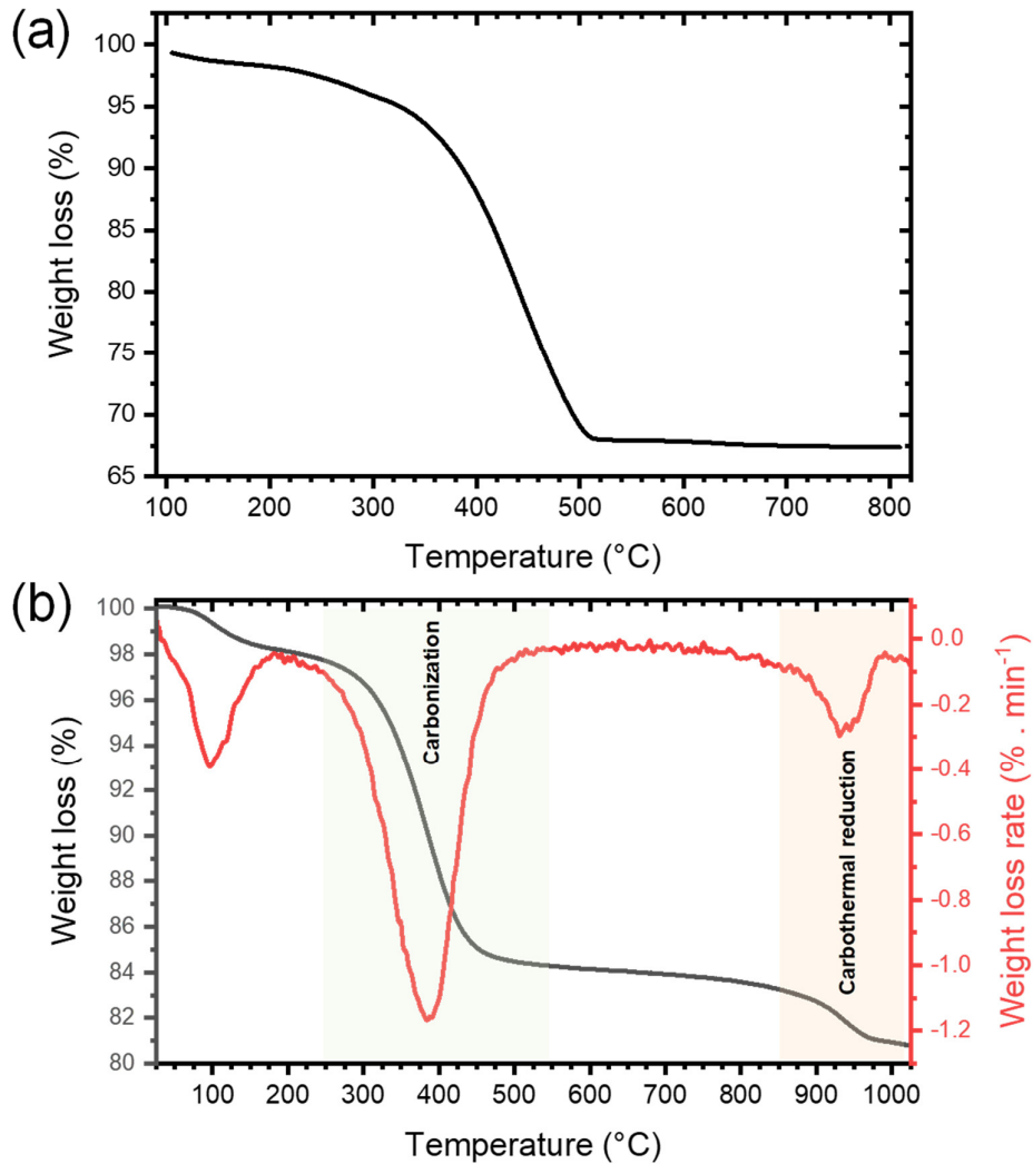
Figure 2. Thermogravimetric analyses performed (a) under synthetic dry air flow (50 mL min -1 ) and (b) under argon flow (50 mL min -1 ) at 10°C min -1 of xer-TiO 2 .
