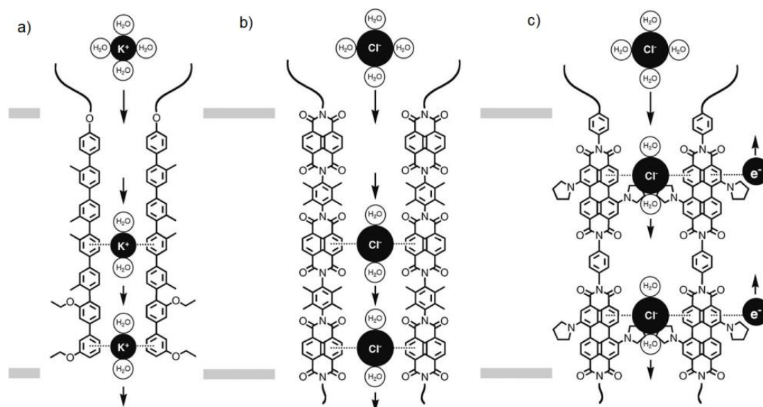
Figure 31. Structures of a) Rigid p-oligophenyl cation- \pi ; b) oligonaphthalenedimide and c) oligoperylene-dimide anion- \pi slides. Adapted with permission from ref. 101. Copyright 2009, Wiley WCH.
