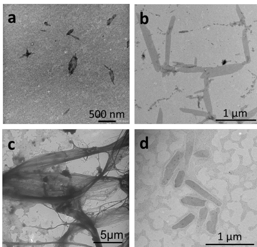
Figure 3. TEM images of self-assembled structures obtained by micellization of 1 \text{ mg mL}^{-1} solutions of the P(VDF- co -HFP)- b -PEG- b -P(VDF- co -HFP) triblock copolymer in (a) DMF, (b) acetone, employing ethanol as a selective solvent for PEG; and (c) DMF, (d) acetone, employing water as the selective solvent for PEG. Final concentration of all samples = 0.14 \text{ mg mL}^{-1} , solvent: selective solvent final ratio = 1:6.
