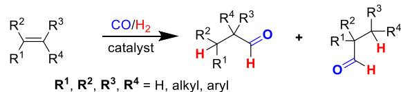
Scheme 20. Hydroformylation, Also Known as Oxo Synthesis or Oxo Process
