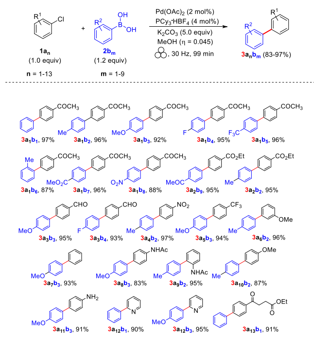
Scheme 3. Examination of Substrate Scope under High-Speed Ball-Milling Conditions. Adapted with Permission from Ref 51. Copyright 2016 American Chemical Society
