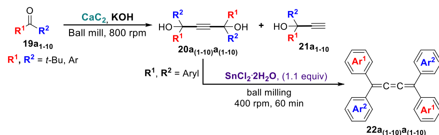
Scheme 25. Alkynylation-Type Reaction in a Ball Mill. Adapted with Permission from Ref 91. Copyright 2019 Wiley-VCH
