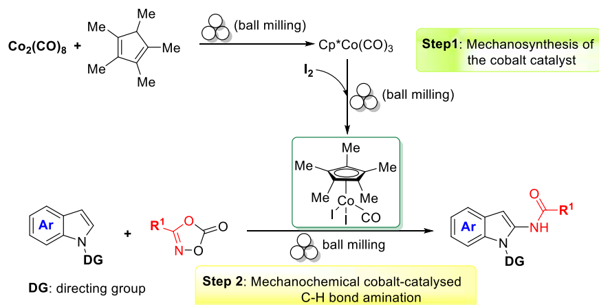
Scheme 29. Mechanochemical synthesis of [\text{Cp}^*\text{Co}(\text{CO})\text{I}_2] and Its Use in C–H Bond Activation by Milling. Adapted with Permission from Ref 98. Copyright 2018 Wiley-VCH
