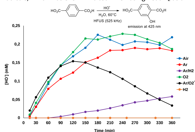
Scheme 3. Titration of \bullet\text{OH} radical using TPA (2 mM) as a function of the gaseous atmosphere. *The decrease in the \bullet\text{OH} radical amount with time under Ar/ \text{O}_2 is due to the large production of \bullet\text{OH} radicals which degrade TPA-OH used as a probe.
