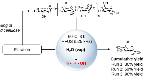
Scheme 1. Depolymerisation of cellulose to glucose induced by HFUS.
