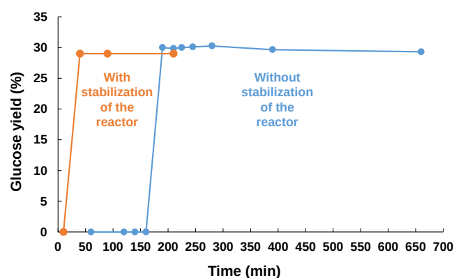
Scheme 2. Kinetic profile of the reaction recorded at 60^\circ\text{C} under air (525 kHz, acoustic power: 0.36 \text{ W}\cdot\text{mL}^{-1} ). Cellulose was introduced before (blue) or after (orange) warm-up of the reactor
