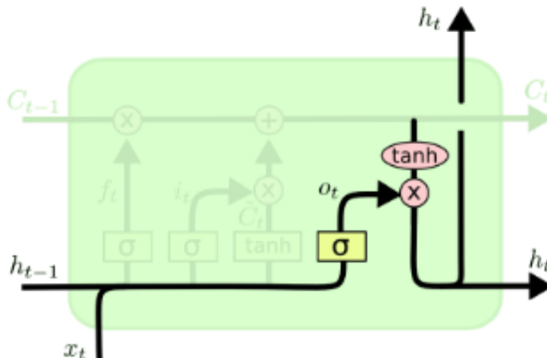
Figure 7: Final step visualization in the LSTM
