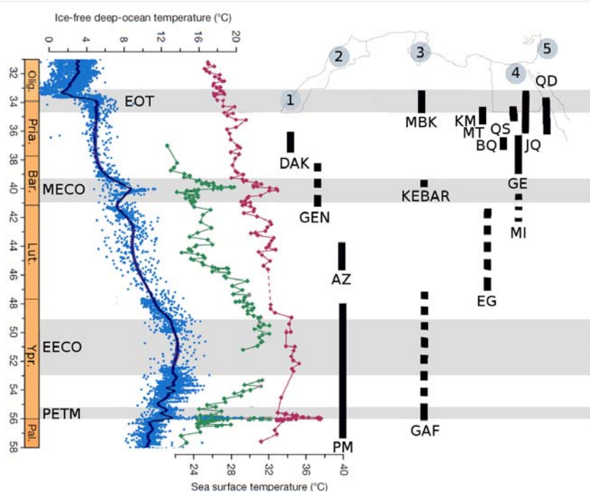
FIGURE 1. Paleotemperatures (ice-free deep-ocean T^{\circ} / tropical sea surface T^{\circ} ) and Thermic events during the “doubthouse” conditions of Eocene period (from Cramwinckel et al., 2018 modified with events dating from Hollis et al., 2019). Stratigraphically and geographical locations of the main deposits with Elasmobranch associations along the southwestern Tethys. Abbreviations: DAK: Dakhla (Adnet et al., 2010), GEN: Genam (Zouhri et al., 2017, in press); AZ: Aznag (Tabuce et al., 2005) PM: Phosphate ores (see Noubhani and Cappetta, 1997), Morocco; GAF: Gafsa basin (see Arambourg, 1952); KEBAR: Kébar (this work and Adnet et al., 2019); MBK: Mabrouk (see Sweydan et al., 2019), Tunisia; EG: ElGedida (see Strougo et al., 2007); KM: KM11 (see Adnet et al., 2011) MT: Minqar Tabaghbagh (see Zalmout et al., 2012); BQ: Birqet Qarun QS: Quar et Sa; GE: Genahamm Fm.; MI: Midawara FM. from Wadi al Hitan, see Underwood et al., 2011), Egypt; QD: Qa Faydat al Dahikya, Jordania, see Mustafat and Zalmout, 2002).
