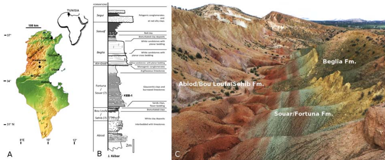
FIGURE 2. Locality of KEB-1, Djebel el Kébar, Kasserine region, Tunisia. A, Simplified topographic map of Tunisia locating the Djebel el Kébar in central Tunisia; B, simplified stratigraphical position of fossiliferous level having yielded the fossil-bearing KEB-1 locality; C, photograph showing the typical badlands of variegated clays from the early Tertiary sequence of Djebel el Kébar. See Merzeraud et al. (2016) for precise details about geological settings.
