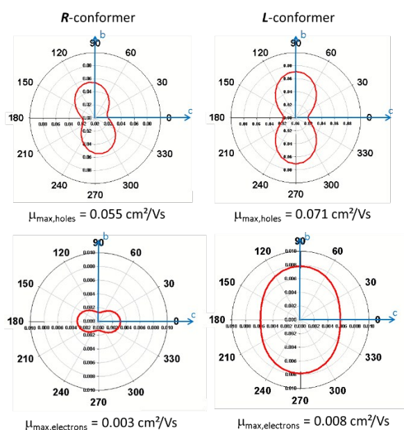
Fig. 17 Anisotropy of the hole (top) and electron (bottom) mobilities (in cm 2 /(V.s)) in the R - (left) and L - (right) conformers of Tp-DMTPS . The horizontal [vertical] direction corresponds to the c -[ b -] unit cell axis. Note that the mobility scale is different for holes and electrons.
