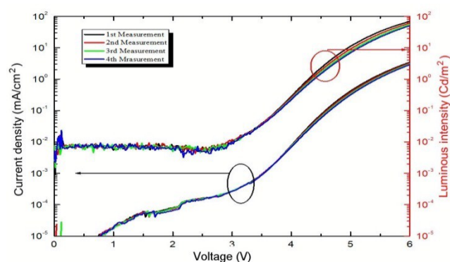
Fig. 14 J-V characteristics and luminous intensity versus voltage of an ITO/PEDOT-PSS/MoO 3 /NPB/Tp-DMTPS/Ca device.
