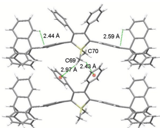
Fig. 3 View of the R -conformers of Tp-DMTTPS in the ab plane showing the methyl C69 nestling between the aromatic rings. Intra and intermolecular CH/ \pi interactions are marked with green dotted lines.
