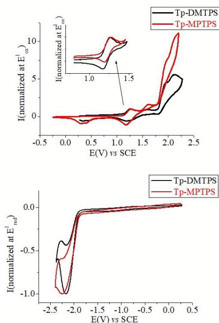
Fig. 12 Top :cyclic voltammetry in \text{CH}_2\text{Cl}_2/\text{Bu}_4\text{NPF}_6 (0.2 M) of Tp-DMTPS (in black) and Tp-MPTPS (in red). Exploration in the anodic direction (top) and in the cathodic direction (bottom). Working electrode: platinum disk, sweep-rate: 100 \text{mV}\cdot\text{s}^{-1} .
