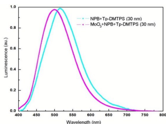
Fig. 13 Normalized EL spectra of Tp-DMTPS .
