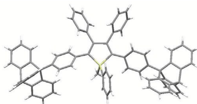
Fig. 4 View of Tp-MPTPS molecular structure.
