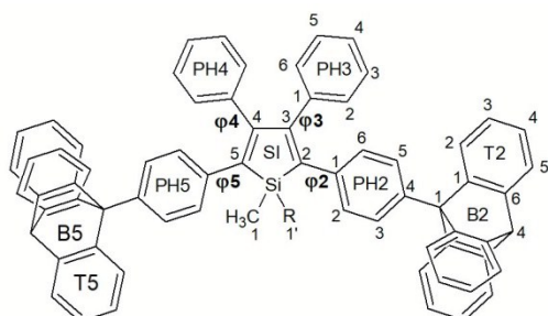
Fig. 1 Labelling scheme for Tp-DMTPS (R 1 ' = Me) and Tp-MPTPS (R 1 ' = Ph).
