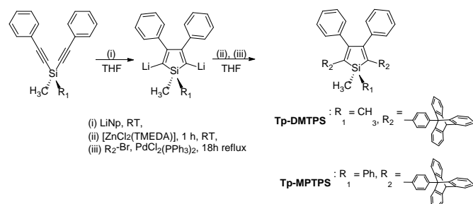
Scheme 1 Synthetic Route to Tp-DMTPS and Tp-MPTPS (see more details in SI).
