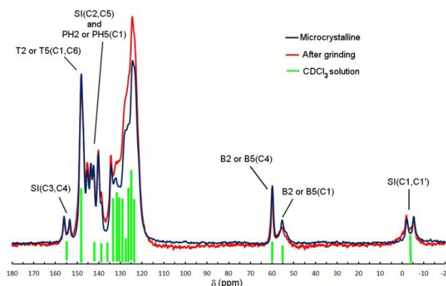
Fig. 11 13 C CP-MAS NMR spectra of Tp-DMTTPS (microcrystalline and ground). Green bars represent the peaks observed in the 13 C{ 1 H} NMR spectrum recorded in CDCl 3 solution. See Fig. 1 for labelling.
