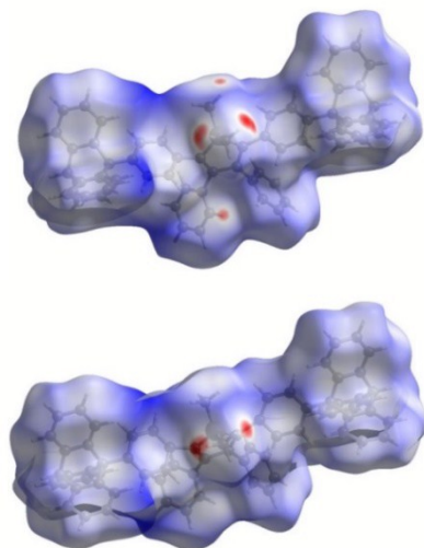
Fig. 5 Hirshfeld surfaces for the L -conformer (top) and the R -conformer (bottom) of Tp-DMTPS .
