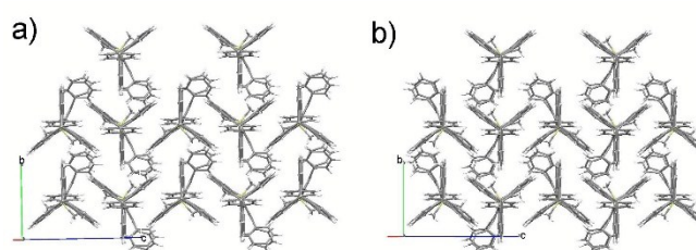
Fig. 2 Views of the crystal packing of Tp-DMTPS showing the triptycene paving in the bc plane for a) R -conformers and b) L -conformers.
