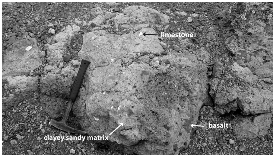
Fig. 6. Matrix-supported breccia bed (debris-flow) from the Lachmine Izayr ejecta embankment.
