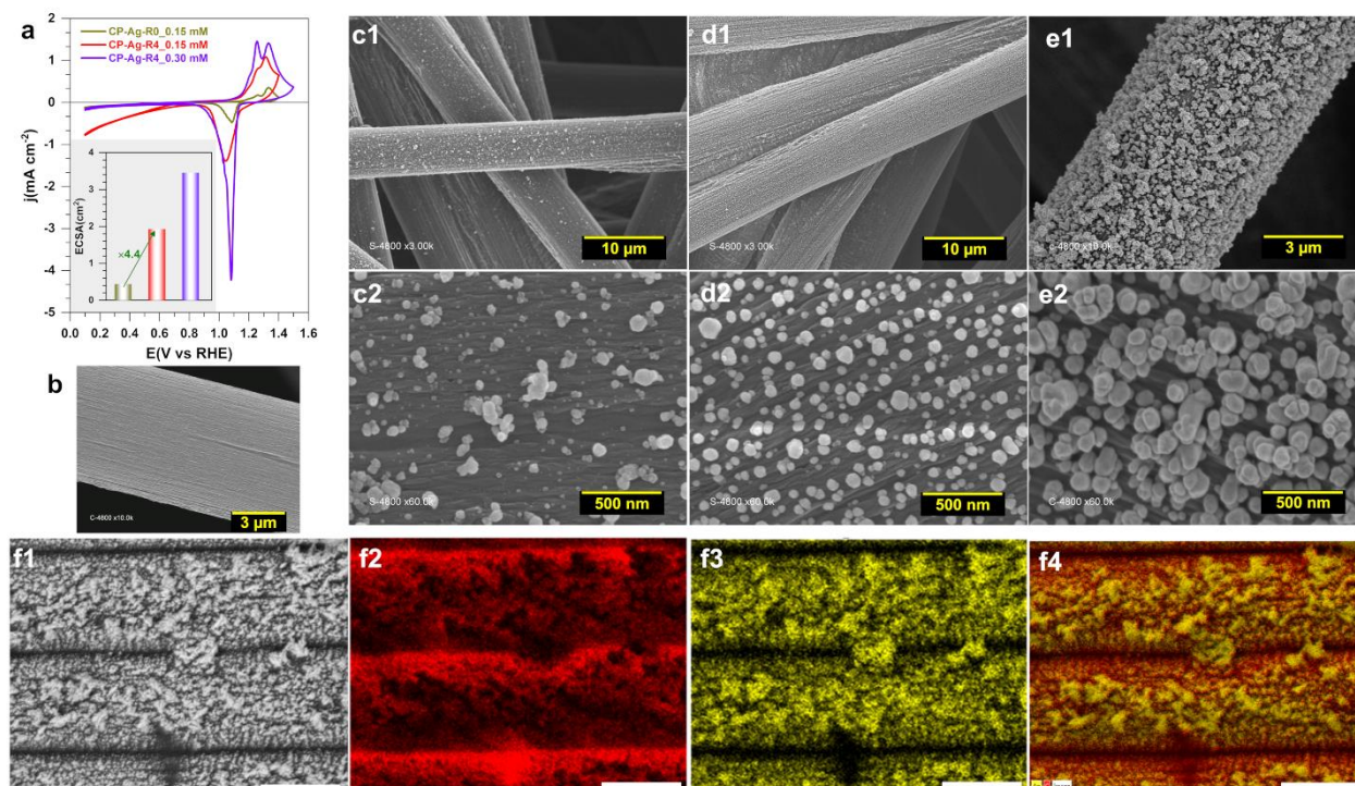
Fig. 1. Characterization of template electrodes. (a) iR-free CVs recorded at 50 \text{ mV s}^{-1} in 1 M KOH and 25 \text{ }^\circ\text{C} (in inset the profiles of the corresponding ECSA) for the as-synthesized materials at \text{AgNO}_3 concentration of 0.15 and 0.30 mM for different ratios R (= n(\text{NH}_4\text{OH})/n(\text{AgNO}_3)) = 0 and 4. SEM micrographs of Ag grown onto a GDE for different ratios: (c1, c2) R = 0 and 0.15 mM \text{AgNO}_3 , (d1, d2) R = 4 and 0.15 mM \text{AgNO}_3 ; (e1, e2) R = 4 and 0.30 mM \text{AgNO}_3 . (f1-f4) SEM and EDX elemental maps (scale bar = 5 \text{ }\mu\text{m} ) for GDE@Ag obtained with R = 4 and 0.30 mM \text{AgNO}_3 : (f2) C, (f3) Ag, (f4) C+Ag.
