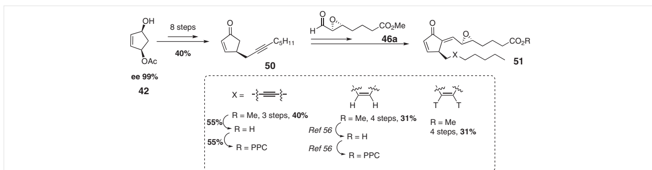
Scheme 11 Modifications for the synthesis of analogues
