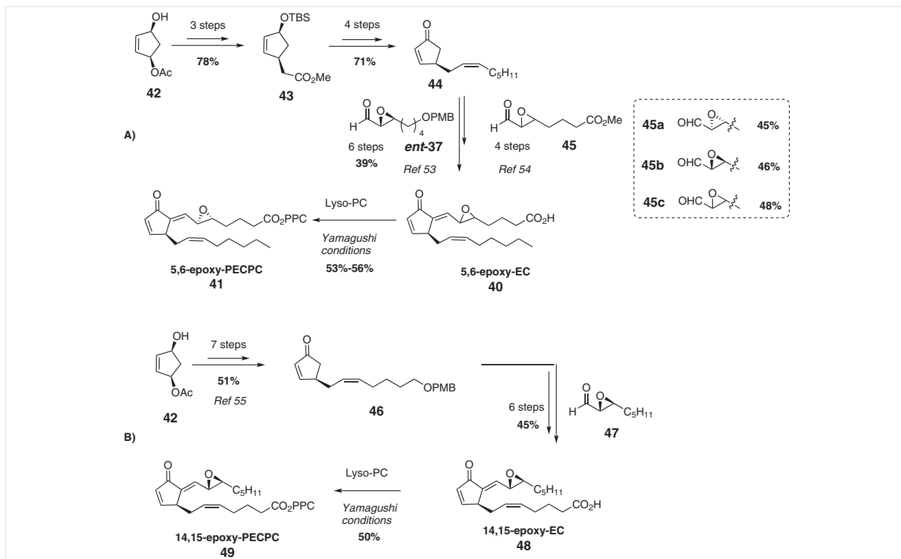
Scheme 10 Synthetic strategy of the Kobayashi group towards A_2 -epoxy-IsoPs
