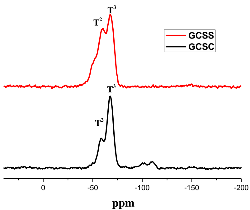
Figure 3: ^{29}\text{Si} OP-MAS NMR spectrum of GCSC and GCSS.
