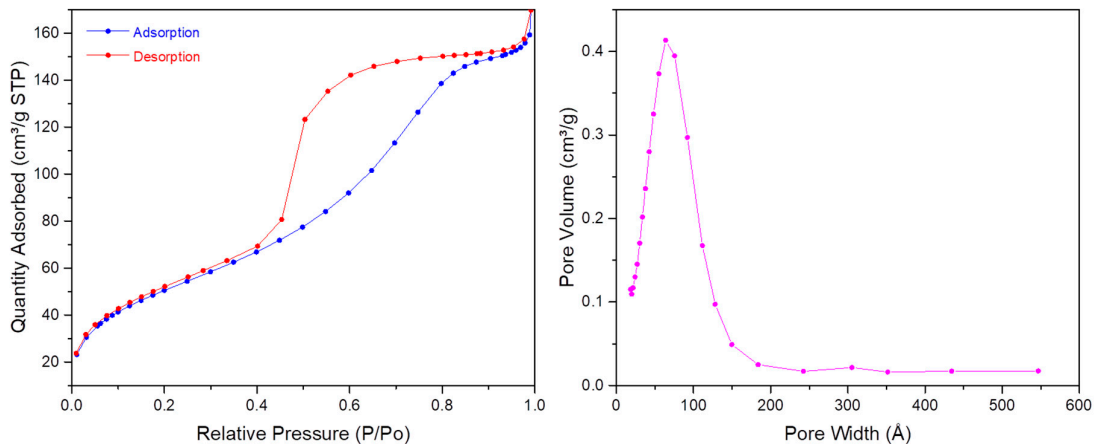
Figure 8. N 2 adsorption–desorption experiments (BET) of P3 PMONPs.
