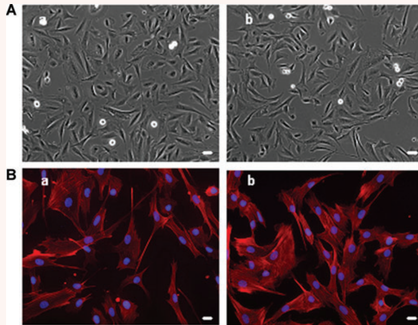
Fig. 2 Comparative morphological analysis of control and FSHD myoblasts. (A) Phase contrast images of a representative control (a; CTL 6) and FSHD (b; FSHD13) myoblast culture showing that FSHD myoblasts have a normal morphology, 10 \times magnification. (B) Observation of actin microfilaments using phalloidin (red) and DAPI (blue) immunostaining on a representative control (a; CTL1) and a representative FSHD (b; FSHD3) myoblast cultures show normal cytoskeleton morphology, 20 \times magnification, bar = 10 \mu m. All these observations were done on the 14 CTL and FSHD myoblast cultures.
