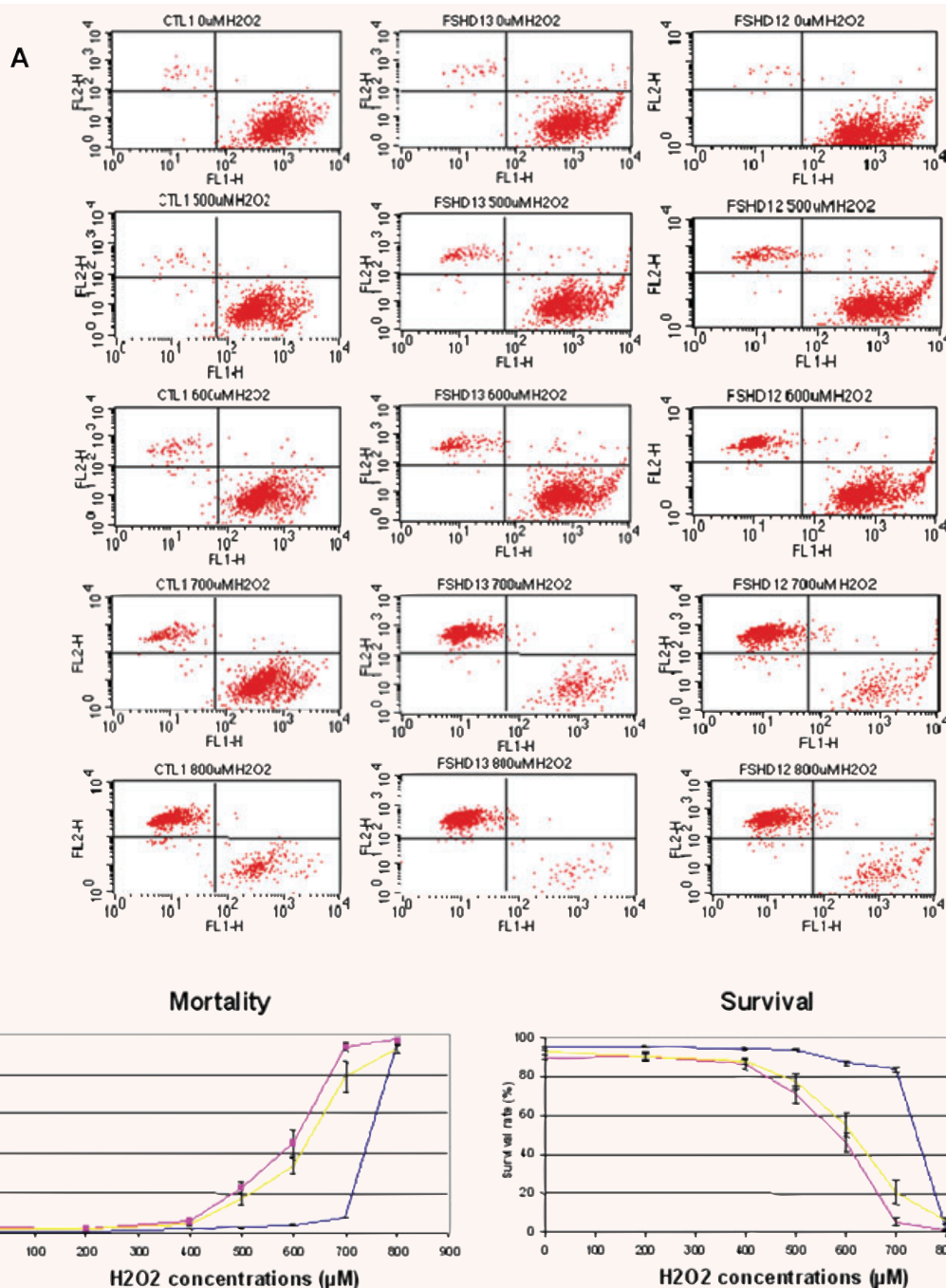
Fig. 4 Comparative analysis of control and FSHD myoblasts response to H_2O_2 -induced oxidative stress. (A) A representative flow cytometry analysis on myoblasts from one control (CTL1), one clinically affected FSHD (FSHD13) and one clinically unaffected FSHD (FSHD12). FACS experiments were conducted on FSHD and control myoblasts after 24 hrs exposure to increasing doses of H_2O_2 . Live cells stained with calcein (green) were sorted with the FL1 channel (down-right window) and dead cells stained with ethidium homodimer-1 (red) were sorted with the FL2 channel (up-left window). (B) Flow cytometry analysis of myoblasts from all control (blue), unaffected FSHD (yellow) and affected FSHD (red). Experiments were performed twice on two independent cultures.
