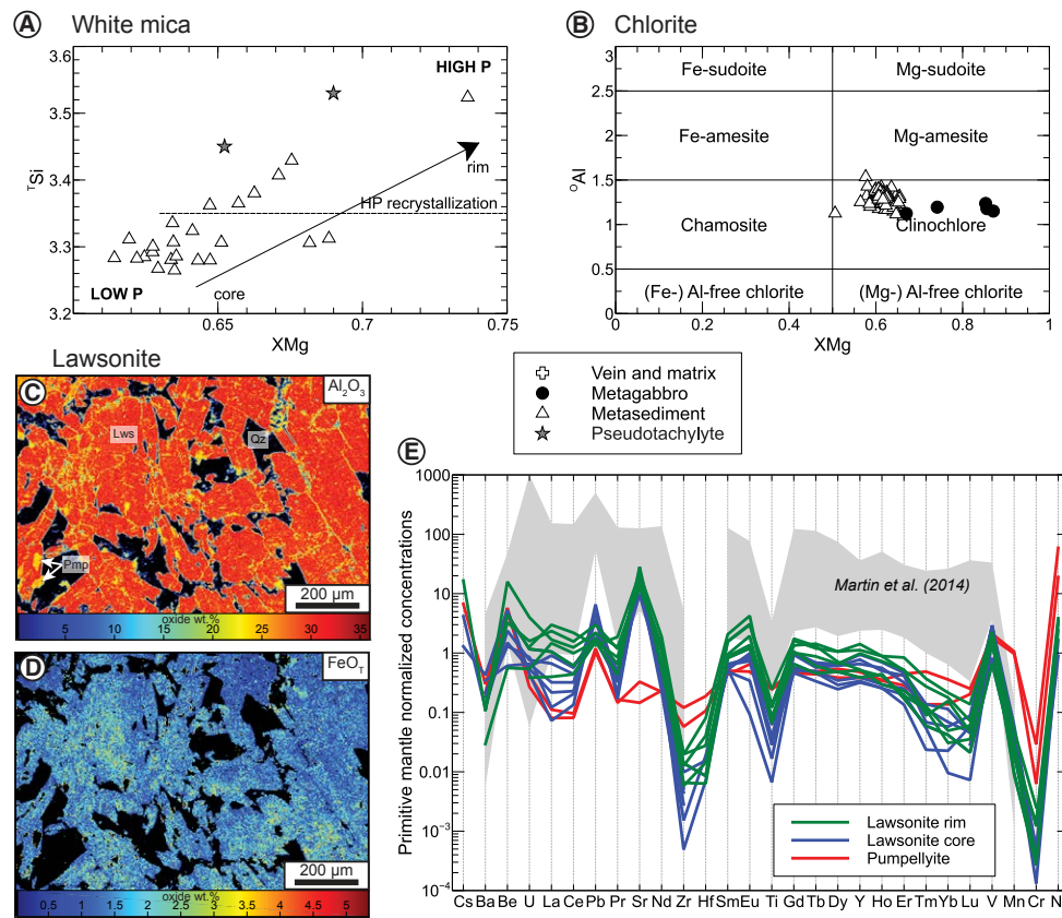
Figure 7. Chemistry of metamorphic minerals. (A) 4 Si versus XMg of white mica; (B) 6 Al versus XMg of chlorite; (C) Al 2 O 3 map of a lawsonite vein (1529); (D) FeO map of lawsonite inside a lawsonite vein (1529); and (E) trace-element patterns of lawsonite in vein.
