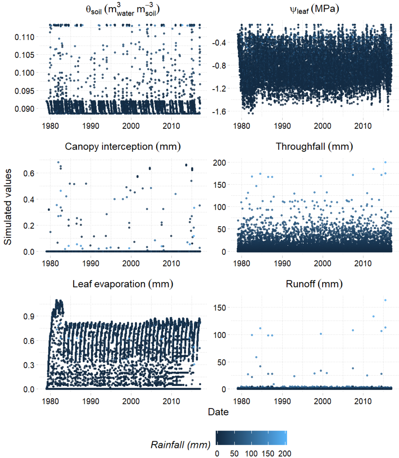
Figure D.2. DynACof outputs related to the water balance at daily time-scale and plot scale for the period starting from 1979-01-01 until 2016-12-31. \theta is the volumetric water content for the full soil profile, and .
