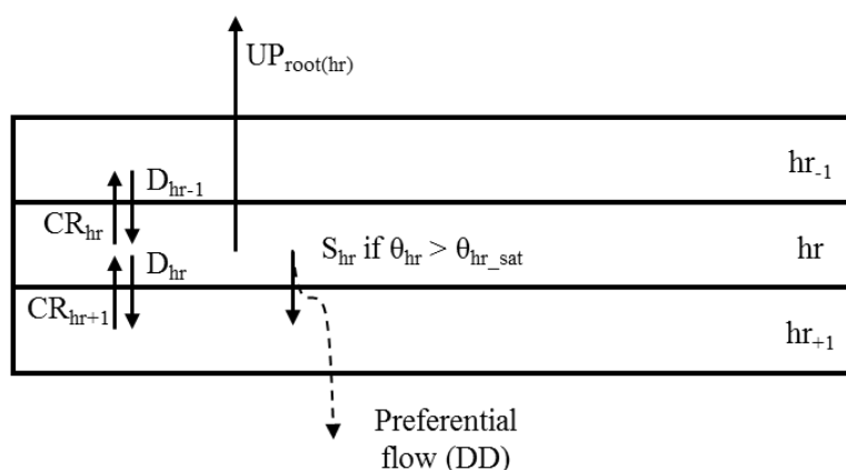
Figure 2: Schematic representation of the water fluxes that modify the water content of a soil horizon hr . The water input fluxes can be the drainage from the upper horizon ( D_{hr-1} ) and the capillary rise from the lower horizon ( CR_{hr+1} ) that depend on the potential gradient between the concerned horizons. The output fluxes are the drainage ( D_{hr} ) and the capillary rise ( CR_{hr} ), the root water uptake ( UP_{root(hr)} ) and the surplus ( S_{hr} ) that appears when the horizon water content exceeds the saturated water content. One part of this latter flux can directly leave the system as deep drainage ( DD ) when preferential flow is considered.
