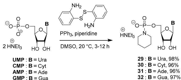
Scheme 14. Synthesis of nucleoside 5'-phosphoropiperidates [66].
