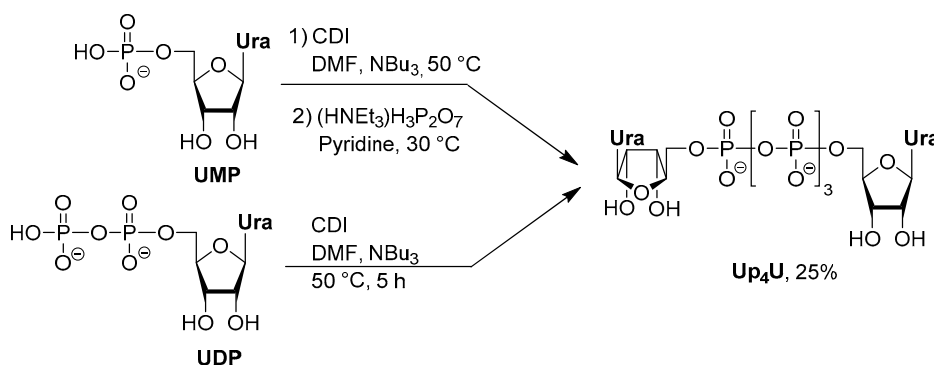
Scheme 3. Dimerization of nucleotides to access symmetrical Up_4U [49,51].
