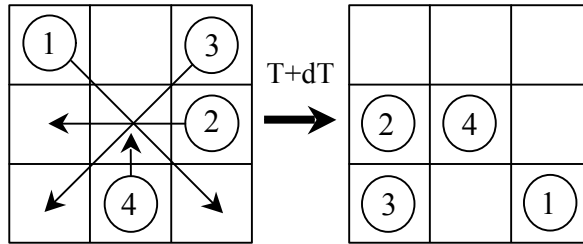
Fig. 3. the problem of action granularity
