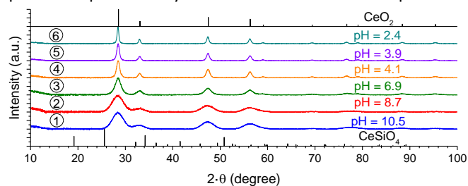
Figure 1. PXRD patterns obtained for samples prepared under hydrothermal conditions (7 days, T = 250^\circ\text{C} ) with starting silicate and cerium(IV) concentrations of 4.2 \times 10^{-2} \text{ mol}\cdot\text{L}^{-1} and initial pH value equal to 10.5 (1), 8.7 (2), 6.9 (3), 4.1 (4), 3.9 (5) and 2.4 (6). Characteristic XRD lines of CeO 2 and CeSiO 4 were extracted from ref 30 and 45, respectively.
