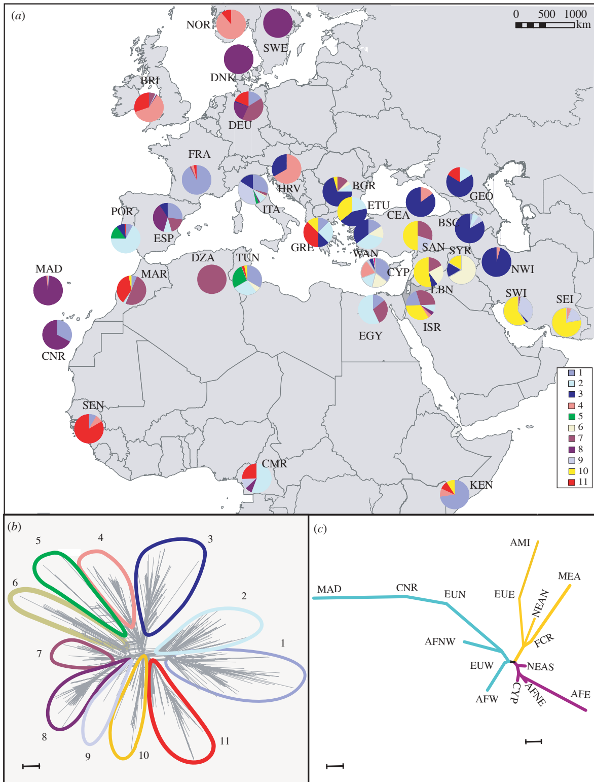
Figure 1. (a) Geographical distribution of the matrilineal haplogroups (HG) according to their position in the network in (b). (b) NeighbourNet network for 1313 individual mitochondrial D-loop sequences. Elliptical envelopes delimitate the 11 HGs considered. (c) Neighbour-joining tree based on Reynolds' distance between regions. Colours help to visualize three main branches roughly reflecting geography. Scale bars, (a) 1–1000 km; (b) 0.0010; (c) 0.05.
