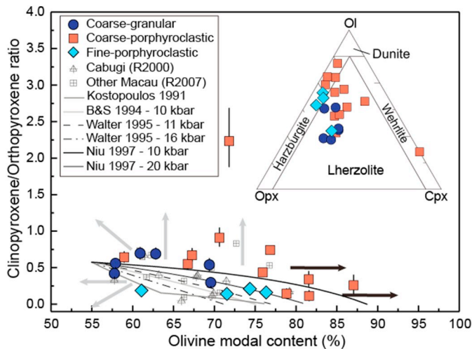
Fig. 7. Modal compositions of the studied peridotites presented as clinopyroxene/orthopyroxene ratio vs. olivine modal content and as the traditional ol-px-cpx ternary diagram (inset). Modal compositions of Cabugi and other Macau volcanics peridotite xenoliths studied by Rivalenti et al. (2000, 2007) are plotted for comparison. Black and gray curves represent the evolution of the modal composition predicted by different partial melting models for an initial fertile modal composition of 55% ol, 28.5% opx, and 16.5% cpx (Baker and Stolper, 1994; Kostopoulos, 1991; Niu, 1997; Walter et al., 1995). Gray arrows indicate evolution trends associated with cpx and/or opx crystallization at the expense of ol (refertilization reactions). Black arrows indicate evolution trends associated with ol crystallization at the expense of pyroxenes (dunitization reactions).
