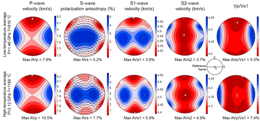
Fig. 12. Average seismic properties for shallow and deep sections of the lithospheric mantle beneath the study area calculated by averaging the elastic constant tensors of the eight low-temperature samples calculated for 916 °C, 1.46GPa and of the nine high-temperature samples calculated for 1189 °C, 2.12GPa. Lower hemisphere stereographic projections presenting the variation of the property as a function of the propagation direction relatively to the structural reference frame (flow direction (X) and normal to the flow plane (Z) shown by the inset). Black squares mark the highest values and white circles mark the lowest ones. Seismic properties data are listed in Table 3 and the elastic tensors, in Supplementary material Table S4.
