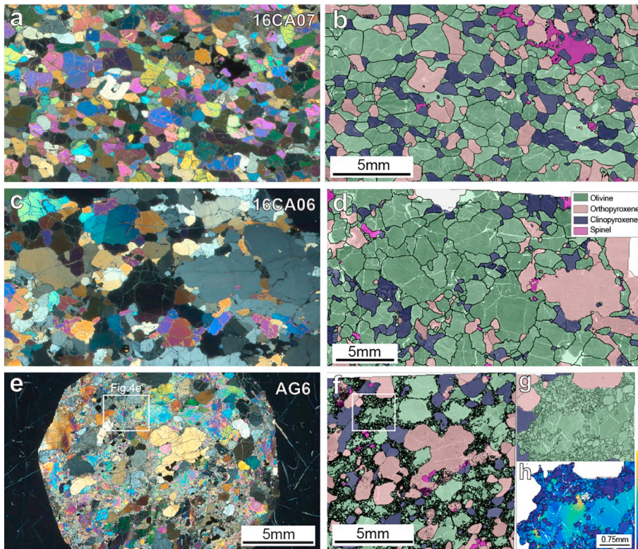
Fig. 3. Typical microstructures of Macau peridotite xenoliths: (a–b) coarse-granular, (c–d) coarse-porphyroclastic, and (e–f) fine-porphyroclastic. (a, c, e) Photomicrographs in cross-polarized light; scale bar is the same in all photomicrographs. (b, d, f, g) EBSD phase maps, which better illustrate the variation in shape of olivine and pyroxenes between the three microstructures. (g) Detail of a partially recrystallized domain in fine-porphyroclastic lherzolite AG6 indicated by the white square in (f). (h) Misorientation relative to the mean orientation of the grain (M2M) map illustrating the difference in intragranular misorientation in olivine between porphyroclasts (high M2M) and neoblasts (low M2M) in the same domain.
