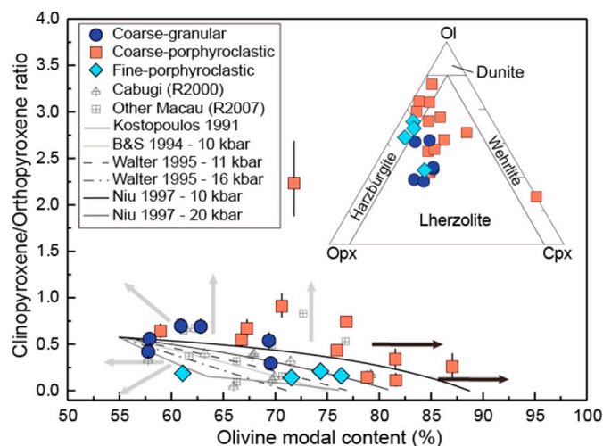
Fig. 7. Modal compositions of the studied peridotites presented as clinopyroxene/orthopyroxene ratio vs. olivine modal content and as the traditional ol-opx-cpx ternary diagram (inset). Modal compositions of Cabugi and other Macau volcanics peridotite xenoliths studied by Rivalenti et al. (2000, 2007) are plotted for comparison. Black and gray curves represent the evolution of the modal composition predicted by different partial melting models for an initial fertile modal composition of 55% ol, 28.5% opx, and 16.5% cpx (Baker and Stolper, 1994; Kostopoulos, 1991; Niu, 1997; Walter et al., 1995). Gray arrows indicate evolution trends associated with cpx and/or opx crystallization at the expense of ol (refertilization reactions). Black arrows indicate evolution trends associated with ol crystallization at the expense of pyroxenes (dunitization reactions).
