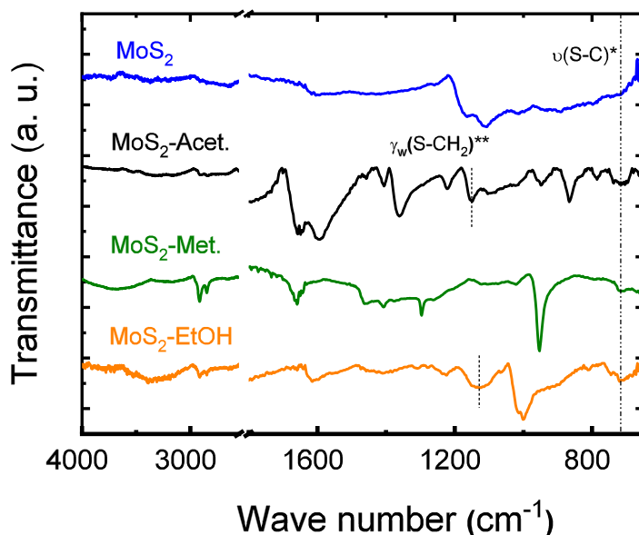
Supplementary Figure 7. ATR-FTIR spectra of pristine (non-functionalized) MoS 2 (blue), acetamide- functionalized MoS 2 (black), methyl- functionalized MoS 2 (green) and ethyl-2-ol- functionalized MoS 2 (orange); (*: 7 ; **: 8 ).
