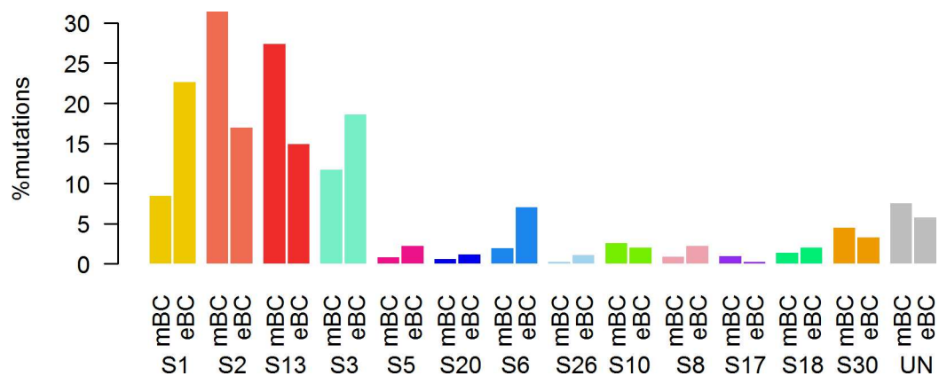
Fig 6. Distribution of the number of mutations according to mutational signatures in HR+/HER2- metastatic and primary (TCGA) breast tumors.
