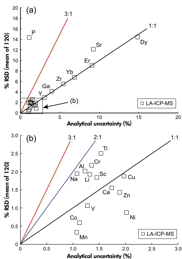
Figure 2. Assessment of homogeneity of olivine Mong-GOL Sh 11-2 on the basis of LA-ICP-MS analyses of 120 individual olivine fragments. Values of homogeneity index of 1 (black lines), 2 (blue line) and 3 (red lines) are shown. (a) The full range of values; note that P is the only element showing substantial heterogeneity. (b) Elements with % RSD values < 3\% . See text for details.
