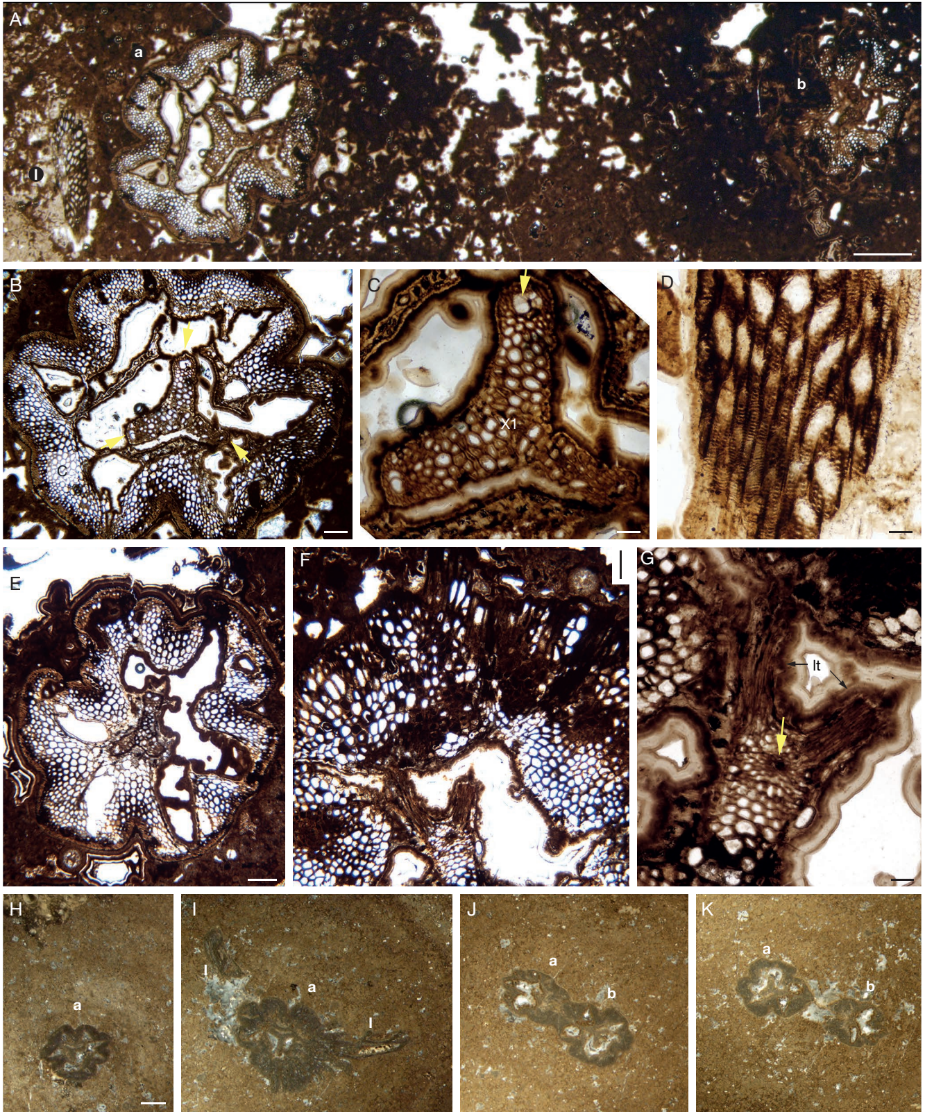
FIG. 4. — Specimen from Coumiac, Montagne Noire, France (MN911): A , slide MN911-A1, general view of the specimen above the level of branching, showing a main axis (a) on the left with a trace to a leaf (l) and a smaller axis (b) on the right; this section corresponds to the level 7 on Figure 7; B , slide MN911-A1, general view of the main axis in transverse section showing the cortex with six lobes and triangular primary xylem (arrows); C , slide MN911-A1, detail of the stele on A ; note the presence of lacunae (arrow) at the extremity of each arm of the stele and the lack of secondary vascular tissues; D , slide MN911-A2, pitting on the primary xylem of an outgoing branch trace; E , slide MN911-A2, general view of the smaller axis shown on A ; note smaller size of the primary xylem compared to B ; F , slide MN911-A2, detail of the largest axis showing outgoing paired vascular traces at the extremity of the arm; G , slide MN911-A2, detail of F showing the protoxylem strand (arrow) and two outgoing traces (lt); H-K , successive sections showing the branching of the axis; H , below the division; I , node with leaves; J , branching; K , branching complete. These photos correspond to the levels 1, 2, 4, and 5 on Figure 7 and to polished surfaces MN911-B1i, MN911-B1s, MN911-B2s, and MN911-B3i. Scale bars: A, H-K, 1 mm; B, E, F, 200 µm; C, 80 µm; D, 50 µm.
