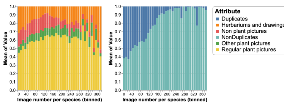
Fig. 4. Average proportion of each noise as a function of the number of training images per species (binned with a step size of 10 pictures)
