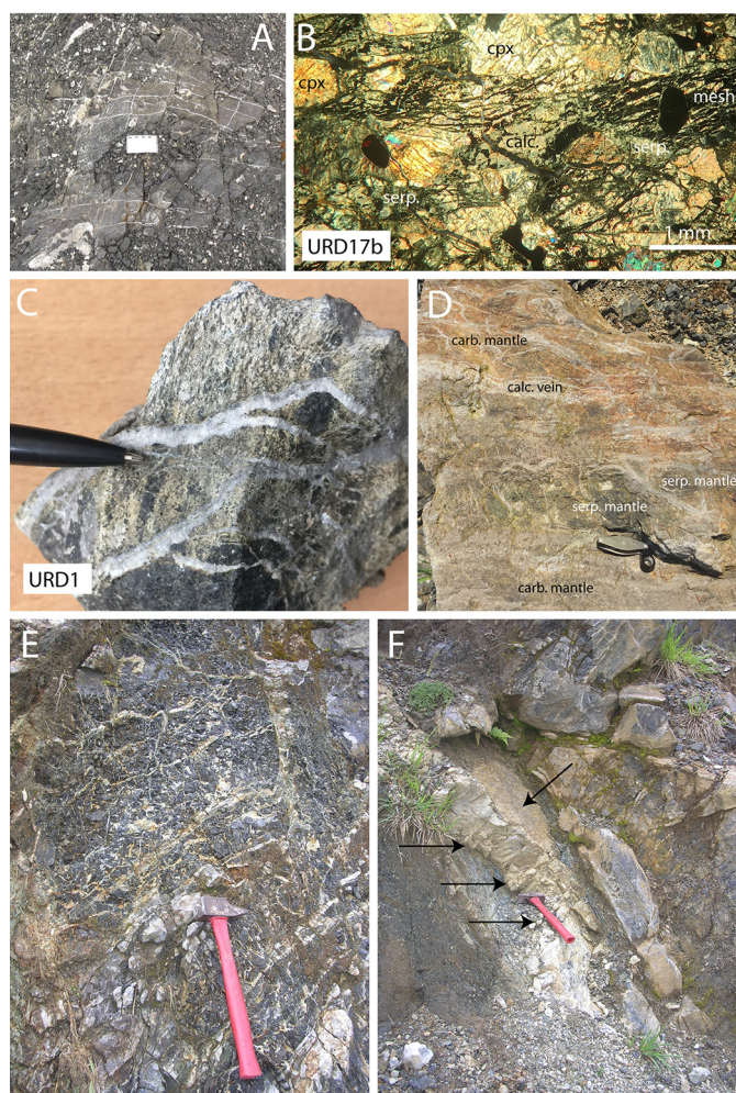
Fig. 8. Ophicalcites at Col d'Urdach and at Bilatre. Field and microscopic aspect. A. Undeformed ophicalcites on the floor of the Col d'Urdach quarry. B. Slightly carbonated mantle lherzolite at the Col d'Urdach “ball trap” section. Note the mesh texture (cpx.: clinopyroxene; serp.: serpentine; calc.: calcite). C. Calcite veining in ophicalcite sample URD1 from the Urdach quarry. D. Alternating carbonated and carbonate-free layers of serpentinitized mantle (Bilatre quarry). E. Multidirectional network of calcite veins (Bilatre quarry). F. Albitite dike (arrows) at the Bilatre quarry in 2007. This outcrops does not exist anymore due to oversampling.
