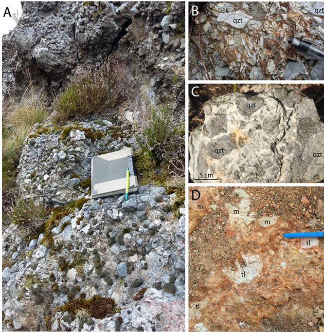
Fig. 5. Photographs showing some typical field aspect of the Urdach breccia. A. General aspect. B. A layer composed of numerous angular clasts of quartzite mylonite. C. Typical aspect of the breccia in the Mer de Her area. Quartzite clasts are cemented by hydrothermal quartz with fluid inclusions of Triassic origin (Nteme, 2017). D. Aspect of the Urdach polymictic breccia near Bilatre (qzt: Ordovician (?) quartzites; m: mylonitic Paleozoic basement; tl: talcified lherzolites).
