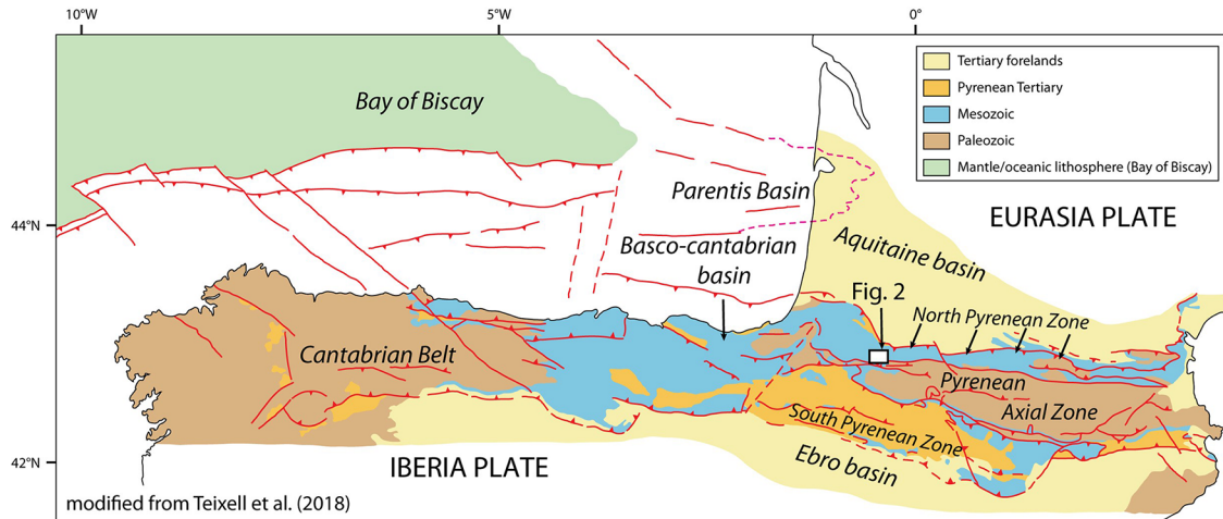
Fig. 1. Simplified structural map of the Pyrenean-Cantabrian belt and location of the study area (modified after Teixell et al. , 2018).
