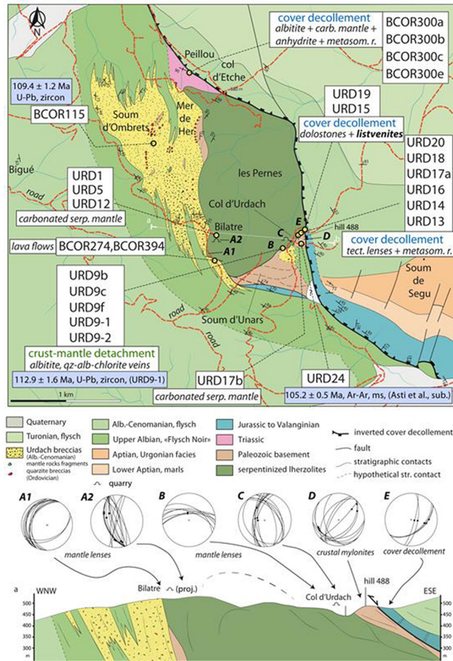
Fig. 4. Detailed geological map of the Urdach massif (Corre, 2017) and corresponding geological cross-section ab. Location of the studied samples. Stereonet D shows the orientation of shear zones and striae in the felsic mylonites of hill 488 (Asti et al. , 2019). Stereonet E shows the orientation of normal faults and associated striae in the “ball trap” section (Urdach cover décollement ) (see faults on Fig. 10).
