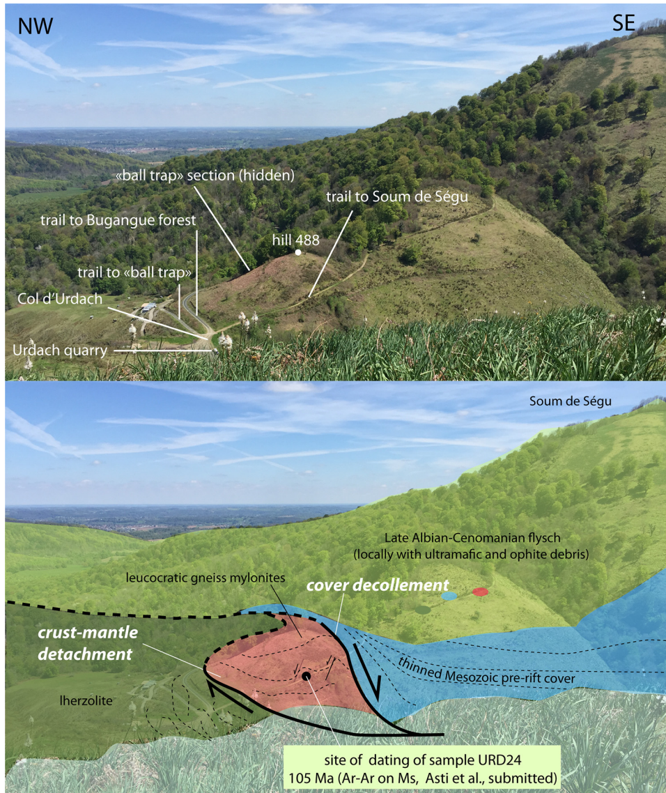
Fig. 6. Geological interpretation of a panoramic view of the Col d'Urdach area taken from the summit of Soum d'Unars looking to the NE. Trails, roads and main fault contacts cited in text are shown.
