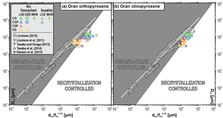
Figure 8. (a) Zener diagram showing average area-weighted olivine grain size ( D_{\text{O1}} ) as a function of grain size and volume fraction of pyroxene ( d_{\text{Px}}/f_{\text{Px}}^{0.52} ) in the Oran mantle xenoliths. Data are plotted considering orthopyroxene (a) and clinopyroxene (b) as secondary phases in the olivine matrix. The diagram shows the transition from second-phase (grey-shaded field) to dynamic recrystallization (white-shaded field) controlled microstructures after Herwegh et al. (2011). Comparative data are from natural peridotite shear zones in the Oman ophiolite (Linckens, 2010; Linckens et al., 2011a, b; Tasaka et al., 2014) and the Josephine peridotite (Hansen et al., 2015), as well as deformation experiments on olivine–pyroxene aggregates (Tasaka and Hiraga, 2013). For plotting the data, a Zener parameter of Z = 0.52 is used following Tasaka et al. (2014), and the solid white line in the background is the fit presented in their work. Abbreviations in the legend are the same as for Fig. 2.
