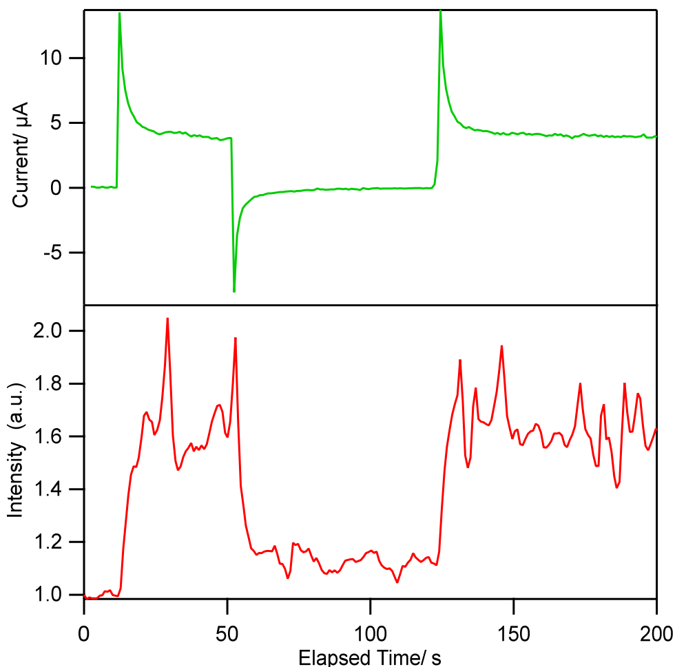
Fig. 9 : A: Bottom (red) : Fluorescence of the TBT recorded in function of the potential applied to the polymer; Top (green) reduction currents (linked to tetrazines reduction). Potential steps between -0.2V(start) and -1.2V (step) and return to the initial -0.2V potential.
