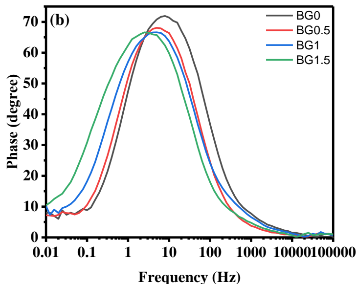
Figure 6. The Nyquist (a) and Bode phase (b) curves of EIS spectra of BG0, BG0.5, BG1 and BG1.5 samples.
