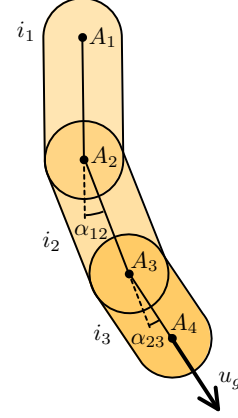
FIG. 2. Root particle geometry and connection between consecutive root elements.
