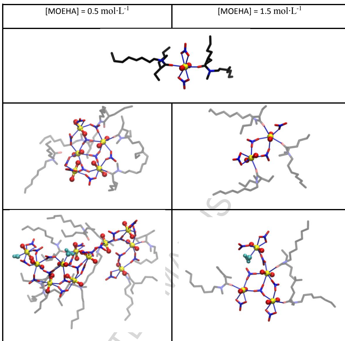
Fig 12 : Representative structures observed in the simulations boxes of MOEHA solutions after extraction of uranyl nitrate. Uranium is yellow, nitrogen is blue, oxygen in red, carbon is black. Hydrogens of DEHBA are not represented. Straight blue lines represent interactions between oxygen and uranium. For a better visibility DEHBA in aggregates are slightly transparent
