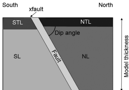
Figure 6. Geometry of the model used in the stochastic inversion. STL—South Top layer, NTL—North Top Layer, SL—South Layer and NL—North Layer. x fault is the prior location of the fault as observed in the field. Model thickness is associated with the thickness investigated by each geophysical method.
