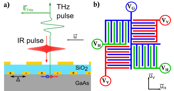
Fig. 1. a) Cut view of an interdigitated photoconductive switch. Interdigitated gold electrodes on top of the GaAs layer consist of 4 μm wide electrodes, equally spaced by a distance Δ = 4 μm. A second metallic layer is composed of metallic fingers covering gaps with a periodicity double that of the first, isolated from the first metallic layer by a 300 nm thick layer of SiO 2 . A femtosecond excitation pulse is focused on the front face of the photoconductive switch generating carriers in the GaAs layer (electrons in blue and holes in red). The THz pulse is emitted from the surface. b) Top view of the intermixed geometry principle (only the first metallic layer is represented). It consists in a pattern made out of two orthogonal small interdigitated photoconductive switches. The pairs of digits share a common ground potential V G , but might be polarized independently with two different electrical potential V H and V V , resulting in respectively horizontal and vertical polarization.
