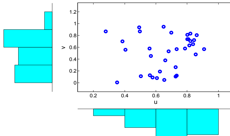
Fig. 11. Cumulative distributions of streamflows at Garbé-kourou (U) and Kandadji (V)
