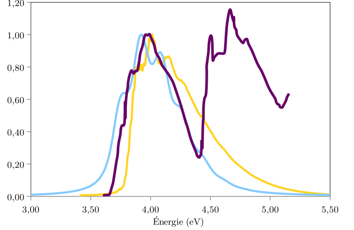
FIG. 13. Theoretical absorption spectra of benzopyran (blue line). Purple line: experimental absorption spectrum of 2,2-diethylchromene (the \text{CH}_2 group is replaced by \text{C}(\text{CH}_2\text{CH}_3)_2 ) at 77 K in 3-methylpentane. In yellow the spectrum with the 12D model of Ref. 40 at the CASSCF level of theory shifted to smaller to lower transition energies.
