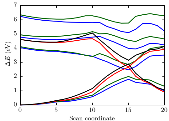
FIG. 5. Comparison between XMCQDPT2 and CASPT2 calculations. The SA-2-CASSCF(12,11)/TVZP curve in black serves as a reference for the XMCQDPT2 calculations, and the SA-2-CASSCF(12,11)/ANO-S-VTZP curve in red for the CASPT2 calculations. The curve MS-4-SA-4-XMCQDPT2(12,11)/TVZP is in blue and the curve MS-4-SA-4-CASPT2(12,11)/ANO-S-VTZP level is in green.
