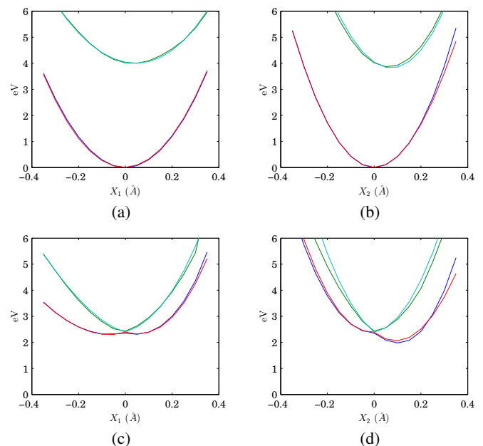
FIG. 12. Cuts through the ab initio and model S_0 and S_1 PESs along the coordinates X_1 and X_2 : in green and blue the ab initio adiabatic energies at the XMCQDPT2 level; in red and light blue the energies given by the model. (a) and (b) are given for FC and (c) and (d) for CI.
