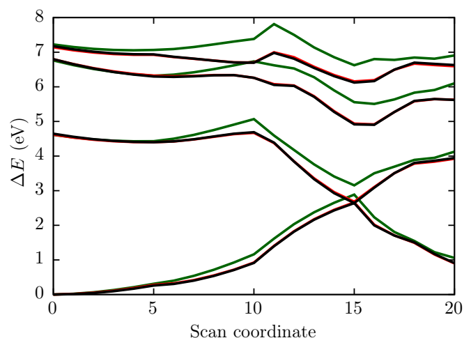
FIG. 2. Comparison of different basis sets on CASSCF calculations: scans with SA-2-CASSCF(12,11)/6-31G* (black), SA-2-CASSCF(12,11)/TZVP (red), and SA-2-CASSCF(12,11)/ANO-S-VTZP (green). The curves present some angular points due to the fact that they are built along four different directions: 0 \rightarrow 5 , 5 \rightarrow 10 , 10 \rightarrow 15 and 15 \rightarrow 20 .
