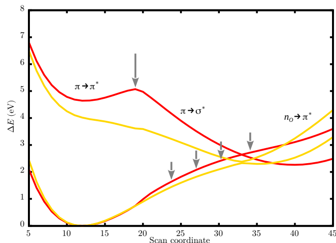
FIG. 7. Comparison between scans with CASSCF and XMCQDPT2 calculations. In red are given the energies at the SA-4-CASSCF(12,11)/TZVP level of theory, in yellow those at the MS-4-SA-4-XMCQDPT2(12,11)/TZVP one. The global S_0 minimum corresponds to x = 12 , the CI minimum to x = 34 (the corresponding geometries are optimized consistently with the levels of theory used for the energies).
