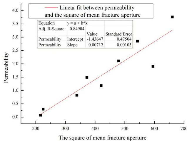
Figure 8. The relationship between permeability and the square of mean fracture aperture of Berea sandstone with an induced fracture.
