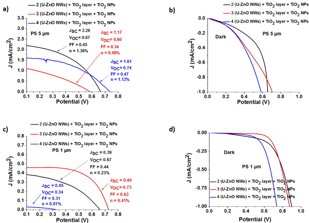
Figure 6. J - V data for DSSCs based on multilayers of U-ZnO NWs covered with a 10nm-thick layer of TiO 2 (ALD) with on top TiO 2 NPs. Each cell was sensitized in dye solution for 12h. Power plots (a) (c) under 500 Wm -2 simulated sunlight, and (b) (d) in the dark. The short-circuit current density ( J_{sc} ), the open-circuit voltage ( V_{oc} ), the fill factor (FF) and the overall photoconversion efficiency ( \mu (%)) are specified for each device.
