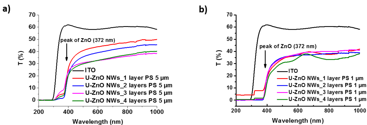
Figure 3. Transmittance spectra of multilayer U-ZnO NWs in function of the PS diameter: a) ~ 5 \mu\text{m} and b) ~ 1 \mu\text{m} .
