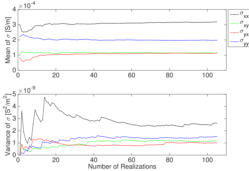
Figure 2. Example showing the calculated mean and variance of the electrical conductivity tensor components \sigma_{xx} , \sigma_{xy} , \sigma_{yx} and \sigma_{yy} , plotted as a function of the number of considered fracture-network realizations for a domain size of 12 \times 12 m. The presented data correspond to Case 12 from Table 1 with \sigma_m/\sigma_f = 10^{-6} . See Section 3 for details.
