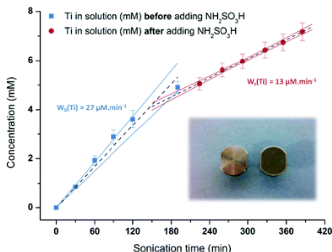
Fig. 5 Titanium (mM) determination (ICP-AES) as a function of sonication time in 1 M \text{HNO}_3 with or without \text{NH}_2\text{SO}_3\text{H} . The black dashed lines are the linear fit of the observed data, and the surrounding lines are assigned to their relative confidence limits. The insert shows pictures of a titanium tip before and after several hours (8–10 h) of sonication.
