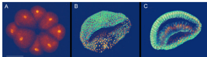
Figure 4: 3D rendering (Amira software) of amphioxus embryos injected with mRNAs coding for fluorescent proteins. Images are extracted from 3D time-lapses acquired on an optimized Leica SP5 2-photon laser-scanning microscope. (A) 16-cell stage embryo expressing nuclear H2B:eGFP. (B) Gastrula stage embryo expressing nuclear H2B:mCherry and the membrane-targeted eGFP:CAAX box. (C) Gastrula stage embryo expressing nuclear H2B:mCherry and the membrane-targeted eGFP:CAAX box. The optical section shows internal cells with nuclear mCherry and membrane-associated eGFP signals. Scale bar = 50 \mu m.
