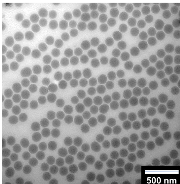
Figure 5. Transmission electron microscopic image of silica particles grafted with poly(vinyl acetate) brushes (PVAc-SiP). The average diameter of the silica particle cores is 130 nm. The number-averaged molar mass of the graft PVAc is 32,200 g/mol.
