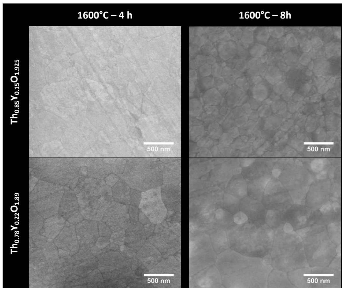
Figure 9. SEM micrographs of Th 0.85 Y 0.15 O 1.925 and Th 0.78 Y 0.22 O 1.89 sintered samples.
