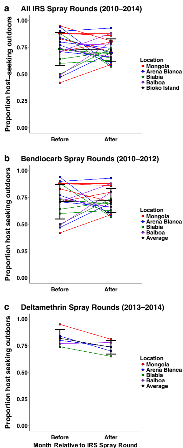
Fig. 5 IRS does not have a direct effect on outdoor host-seeking proportions in months surrounding IRS spray rounds. a Outdoor host-seeking proportions in the month before an IRS spray event and the month after an IRS spray event from 2010 to 2014. Data separated to compare outdoor host-seeking proportions while b bendiocarb or c deltamethrin insecticides were utilized as the IRS insecticide
