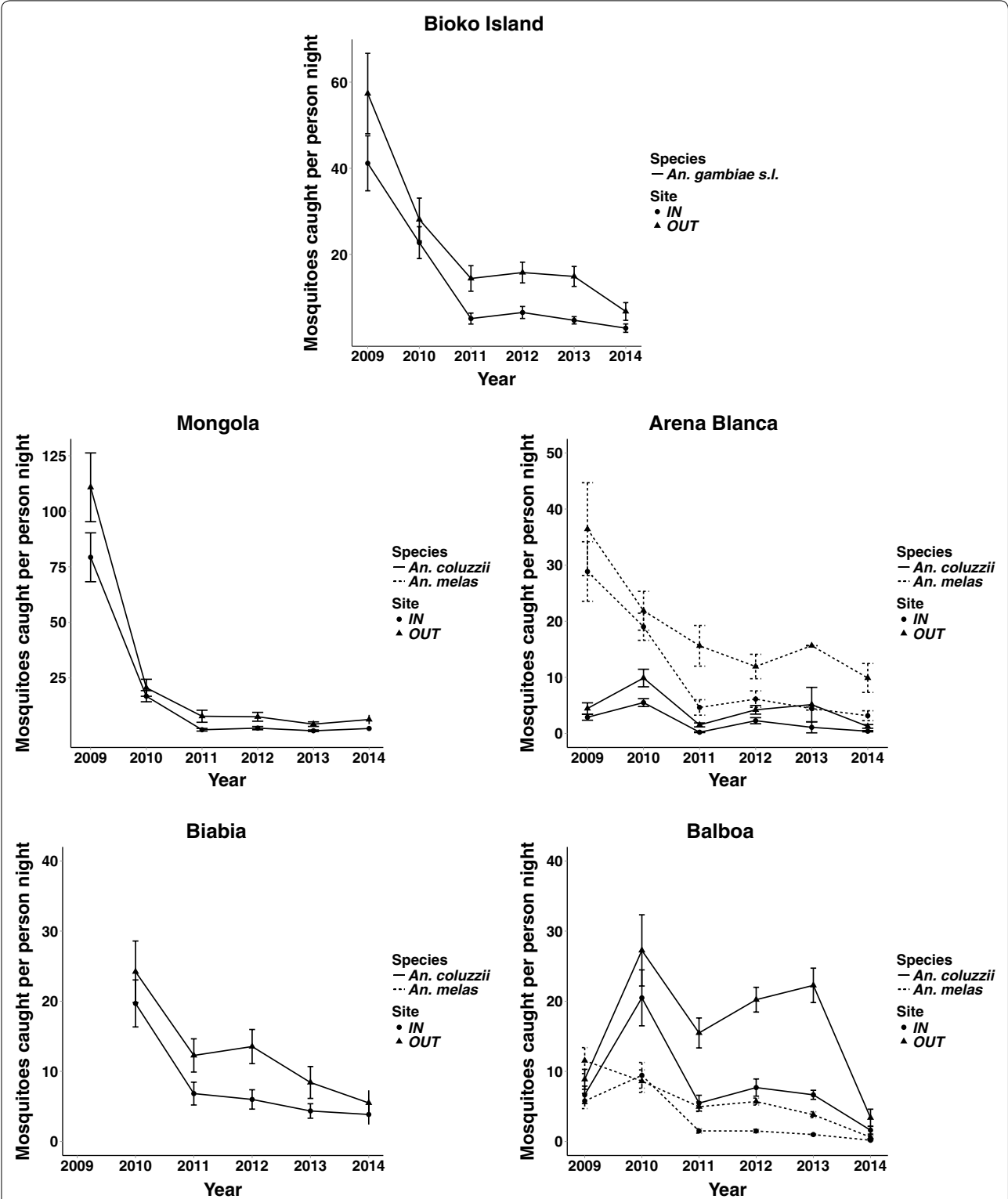
Fig. 2 Indoor and outdoor Anopheles mosquito collection rates decline on Bioko Island from 2009 to 2014. HLC collection rate of An. coluzzii and An. melas from indoor and outdoor sites in Mongola, Arena Blanca, Biabia, Balboa and the average rate across the island. Anopheles coluzzii and An. melas species-specific collection rates are extrapolated from sub-sample of molecularly identified samples. Data presented as mean and standard error
