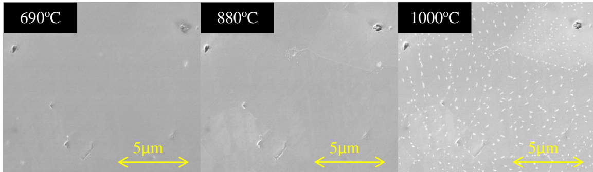
Figure 3. Three micrographs at increasing time/temperature intervals of an LSCF sample annealed in pure O 2
