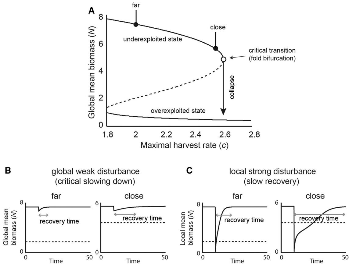
Figure 2. Collapse of resource biomass under increasing harvesting, and two distinct disturbance-recovery experiments in a spatially continuous ecosystem. A Bifurcation diagram of resource biomass. Increasing harvest rate c pushes the resource (mean biomass) toward the tipping point to overexploitation. Continuous lines indicate the two alternative equilibria. The dashed line indicates the unstable equilibrium that divides the two alternative basins of attraction. B We performed a weak global disturbance (by removing 10% of standing biomass) far ( c = 2 ) and close ( c = 2.55 ) to the transition and monitored an increase in recovery time due to critical slowing down. C We performed a strong local disturbance (by removing all standing biomass in an area comprising 1% of the landscape) far ( c = 2 ) and close ( c = 2.55 ) to the transition and monitored an increase in recovery time. Note this increase is not strictly due to critical slowing down. Dashed horizontal lines indicate the threshold between the basins of attraction of the two alternative states. For all simulations, dispersal rate is low ( D = 2.5 \text{ m}^2 \text{ day}^{-1} ).
